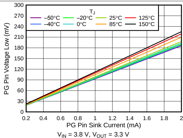
Figure 17. V_{OL}(PG) vs PG Pin Sink Current
