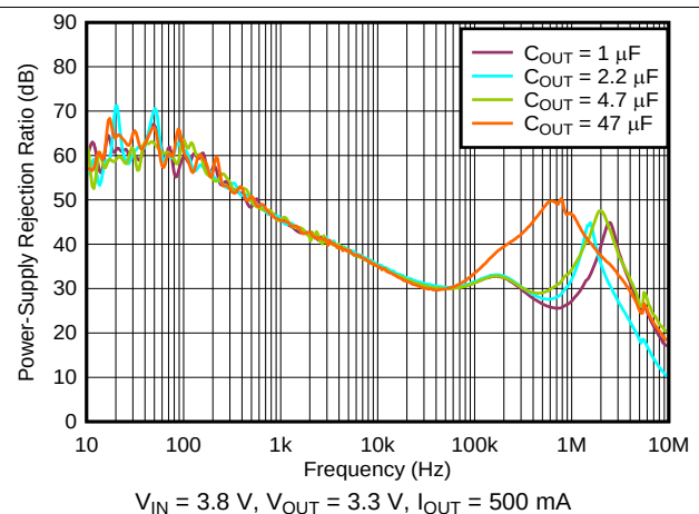
Figure 36. PSRR vs Frequency and C_{OUT}
