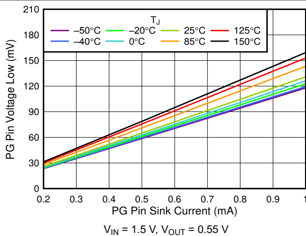
Figure 6-23. V_{OL(PG)} vs PG Pin Sink Current
