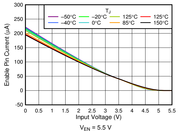
Figure 6-28. I_{EN} vs V_{IN}
