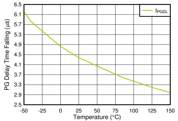
Figure 6-26. t_{PGDI} vs Temperature
