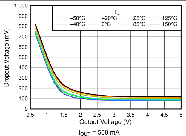
Figure 6-12. V_{DO} vs V_{OUT}
