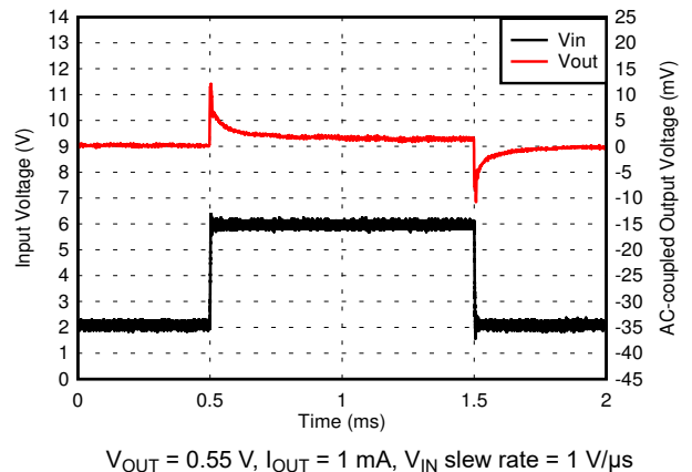
Figure 6-30. 0.55-V Line Transient
