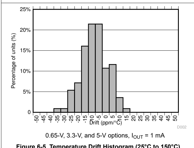
Figure 6-5. Temperature Drift Histogram (25°C to 150°C)
