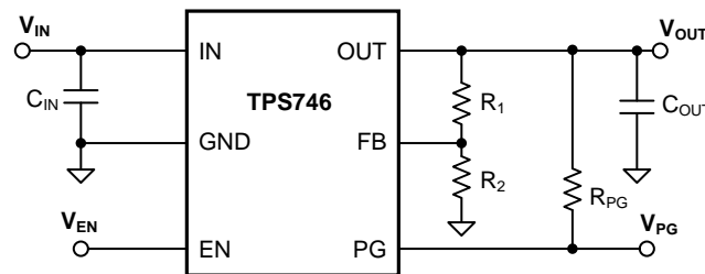
Figure 46. Adjustable Operation
