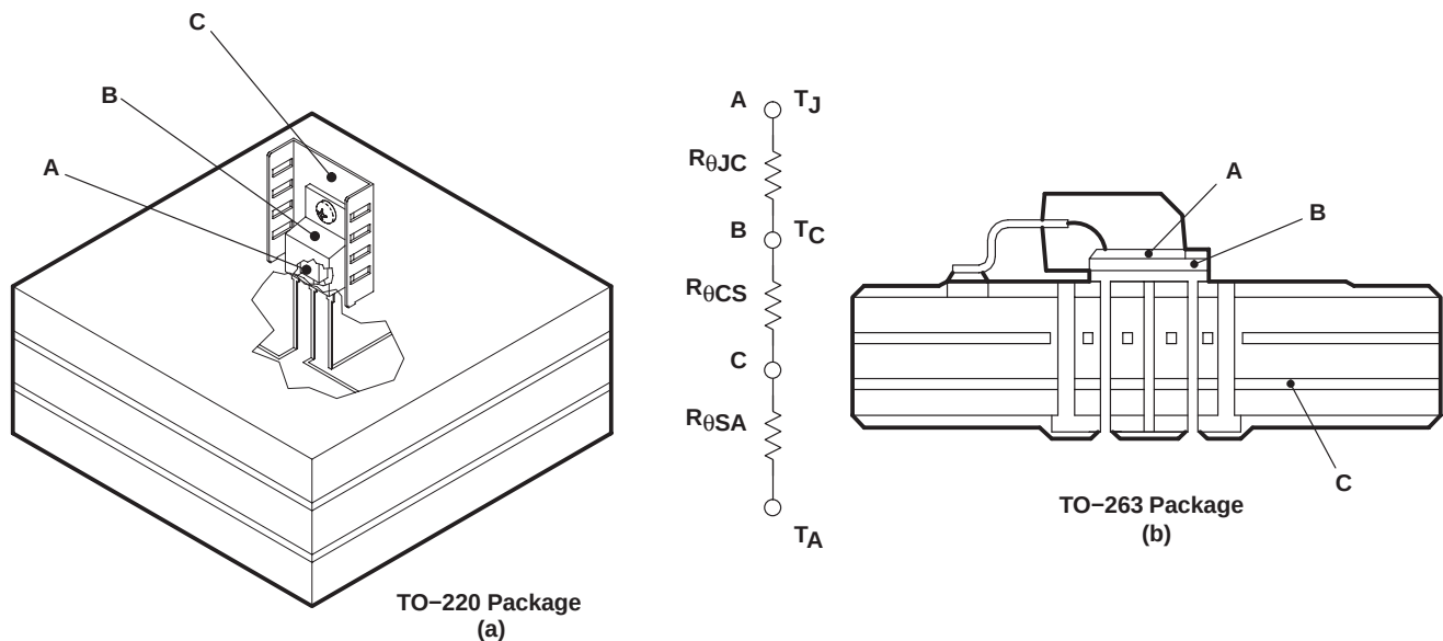
Figure 21. Thermal Resistances
