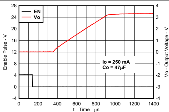
Figure 5-41. TPS76633 Output Voltage vs Time (Legacy Chip)
