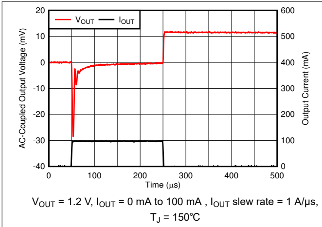
Figure 6-49. Load Transient
