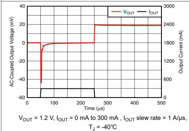
Figure 6-51. Load Transient
