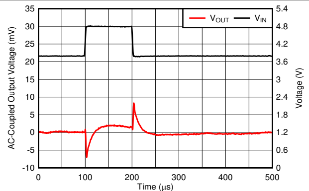
V_{OUT} = 3.3\text{ V} , I_{OUT} = 50\text{ mA} , slew rate = 1\text{ V}/\mu\text{s} , T_J = -40^\circ\text{C}
