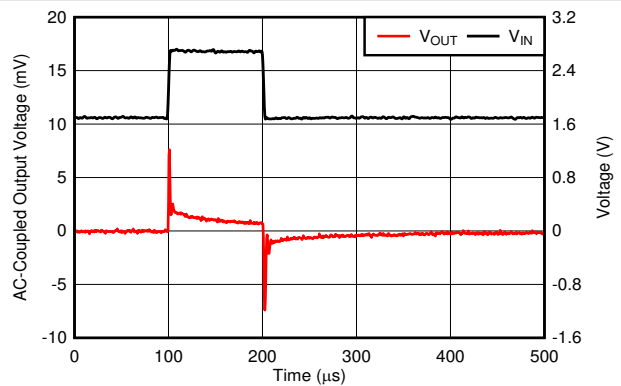
V_{OUT} = 1.2\text{ V} , I_{OUT} = 300\text{ mA} , slew rate = 1\text{ V}/\mu\text{s} , T_J = 25^\circ\text{C}
