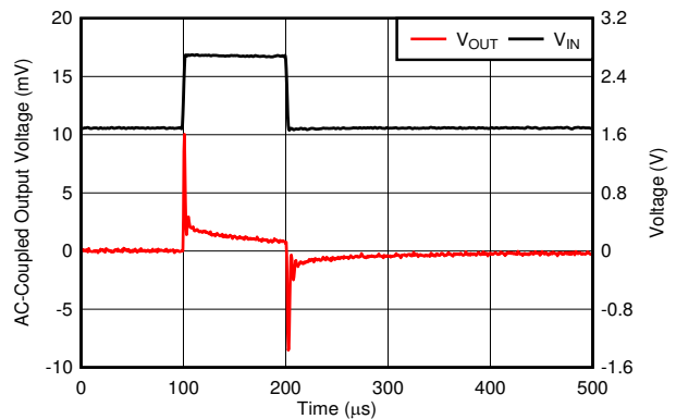
V_{OUT} = 1.2\text{ V} , I_{OUT} = 300\text{ mA} , slew rate = 1\text{ V}/\mu\text{s} , T_J = 150^\circ\text{C}
