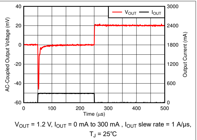
Figure 6-50. Load Transient
