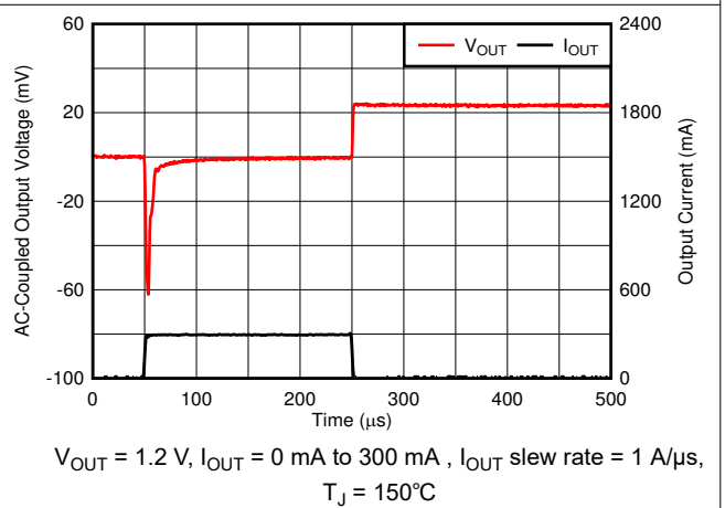
Figure 6-52. Load Transient
