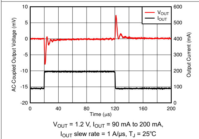
Figure 6-53. Load Transient
