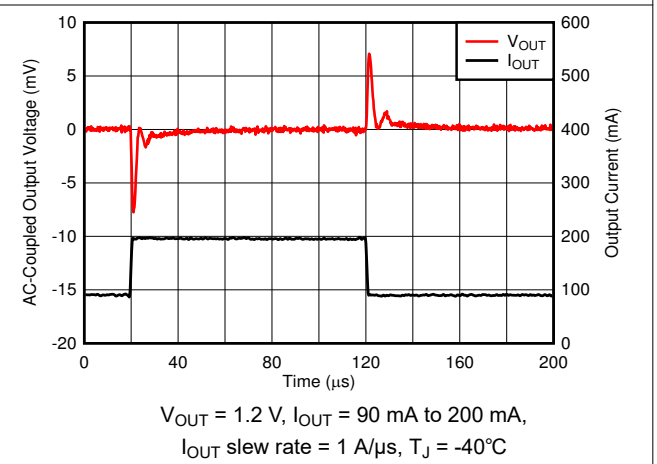
Figure 6-54. Load Transient
