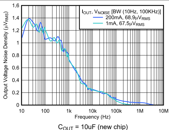
Figure 5-11. TPS793 Output Spectral Noise Density vs Frequency
