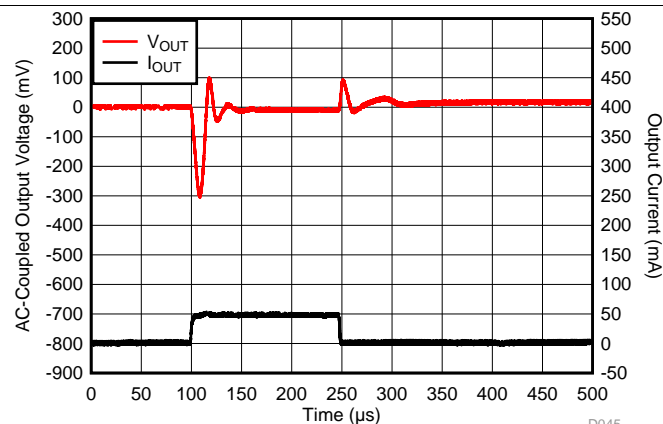
Output current slew rate = 50 mA/µs
