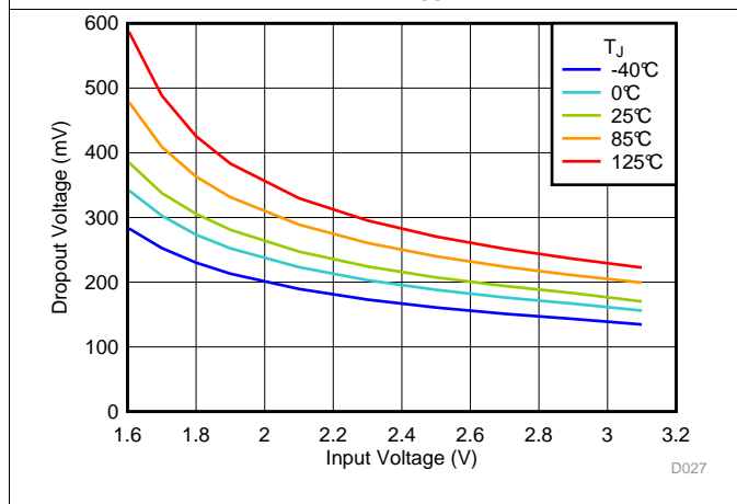
Figure 23. Dropout vs V_{IN} and Temperature
