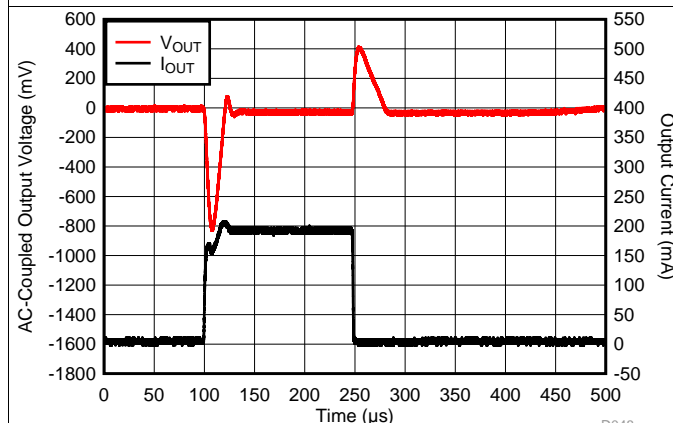
Output current slew rate = 200 mA/µs
