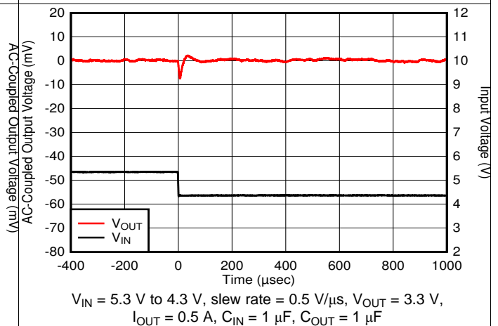
Figure 30. Line Transient
