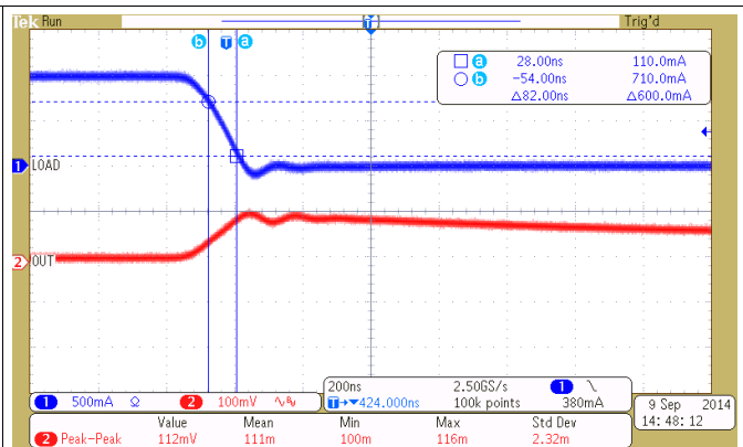
Figure 26. 1-A Load, Expanded View (High to Low), Slew Rate = 7.3 A/μS
