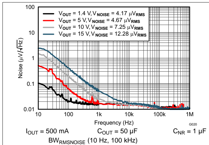
Figure 1. Noise vs Output Voltage
