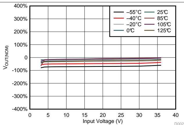
Figure 2. Line Regulation
