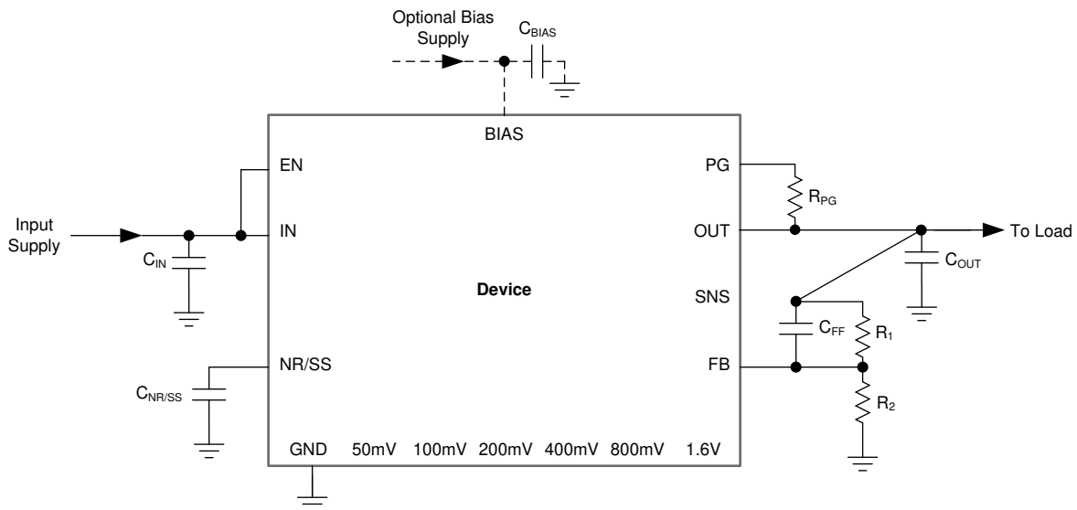
Figure 8-4. Adjustable Operation
