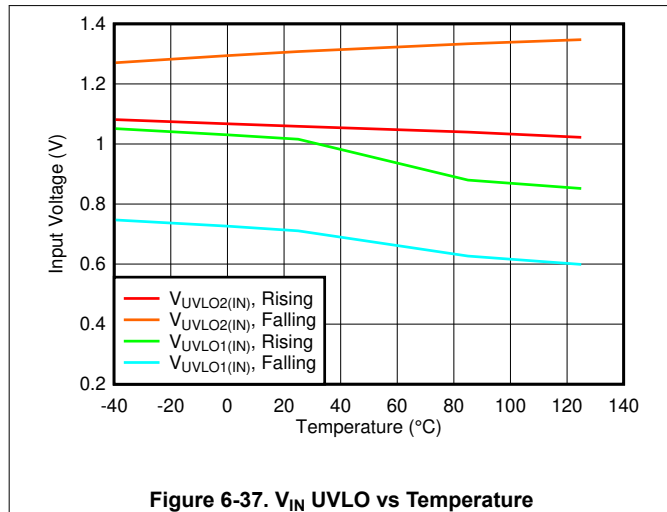
Figure 6-37. V_{IN} UVLO vs Temperature
