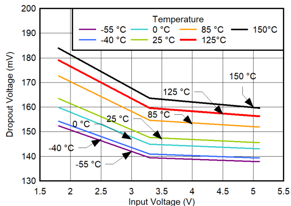
Figure 6-41. Dropout Voltage vs V_{IN} for I_{OUT} = 1\text{ A}
