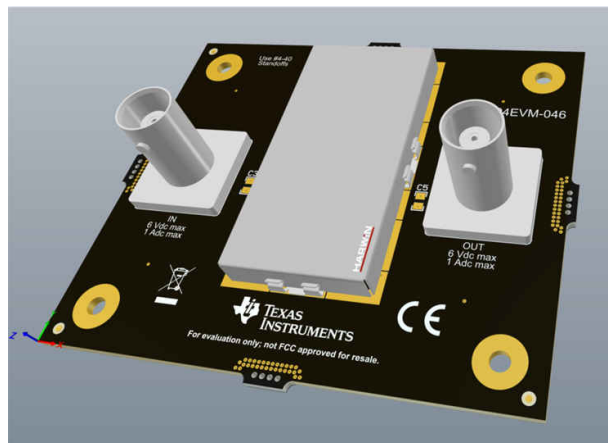
Figure 8-24. TPS7A94EVM-046 3D View
