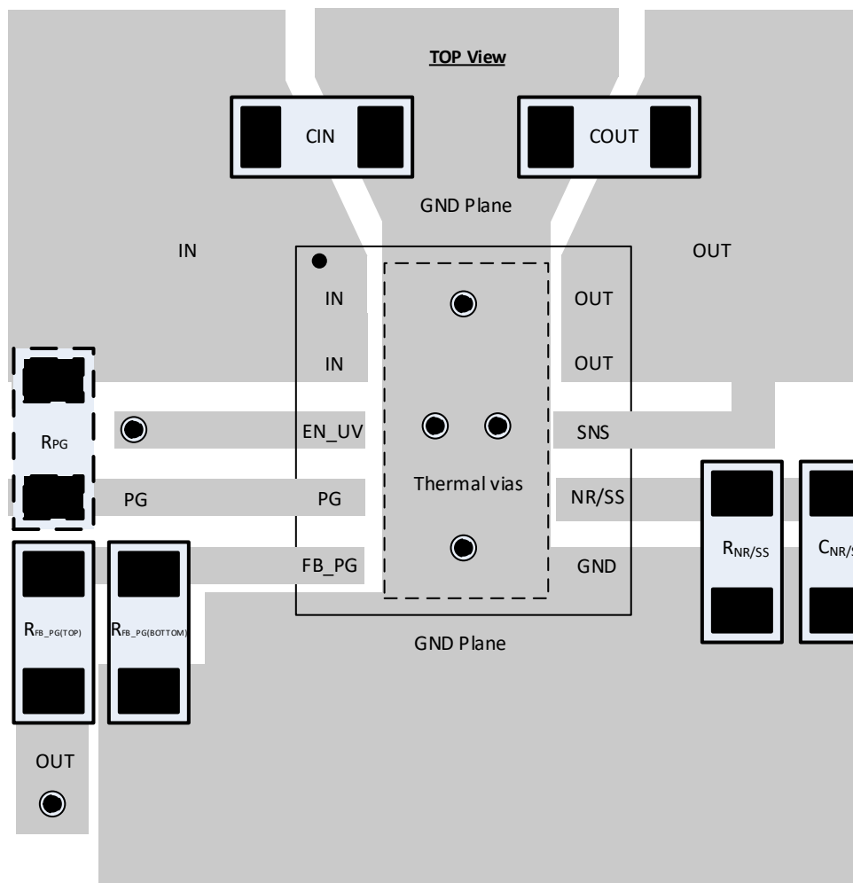
Figure 8-34. Example Layout
