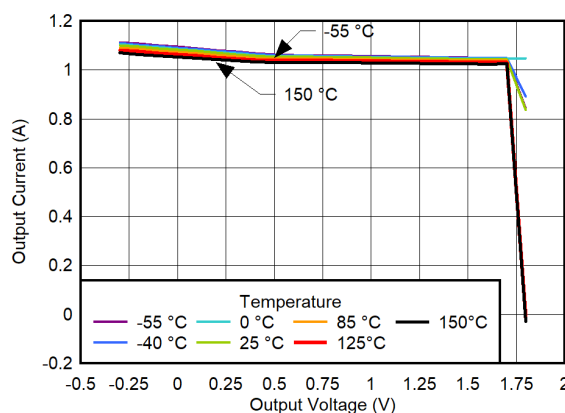
Figure 6-88. 80% Current Limit vs Temperature for V_{OUT} = 1.8\text{ V}
