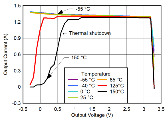
Figure 6-85. 100% Current Limit vs Temperature for V_{OUT} = 3.3\text{ V}
