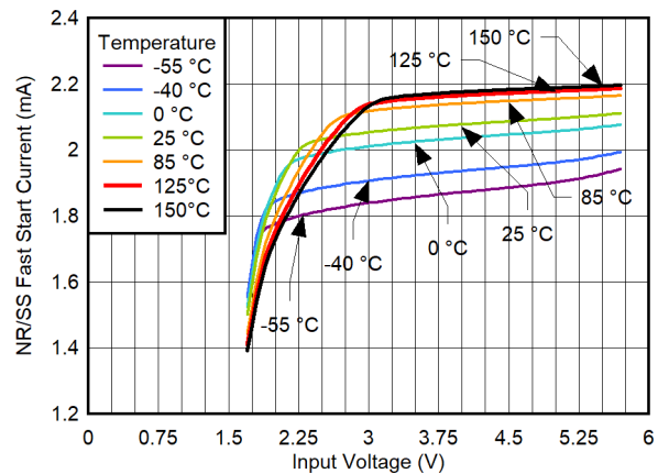
Figure 8-12. I_{FAST\_SS} Reference vs Input Voltage and Temperature for V_{OUT} = 3.3 V
