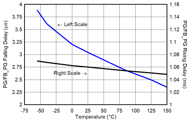
Figure 6-103. FB_PG to PG Pin Rising and Falling Delay vs Temperature
