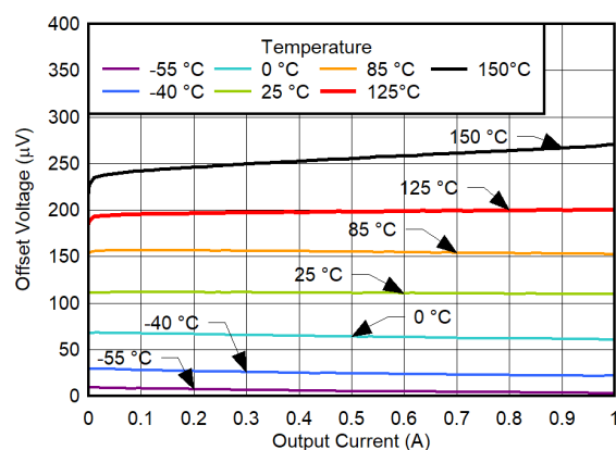
Figure 6-54. V_{OS} vs I_{OUT} and Temperature for V_{IN} = 1.2\text{ V}
