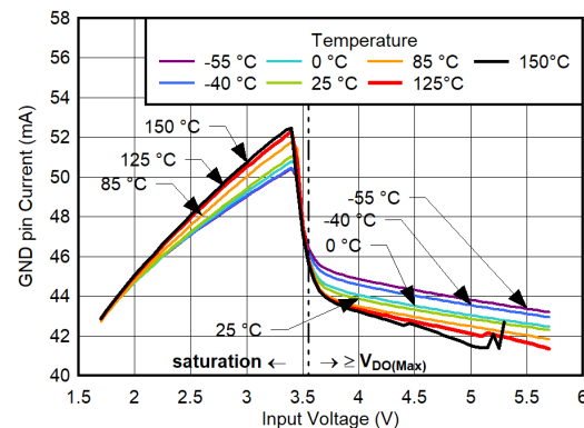
Figure 6-76. GND Pin Current vs V_{IN} and Temperature for I_{OUT} = 1\text{ mA}
