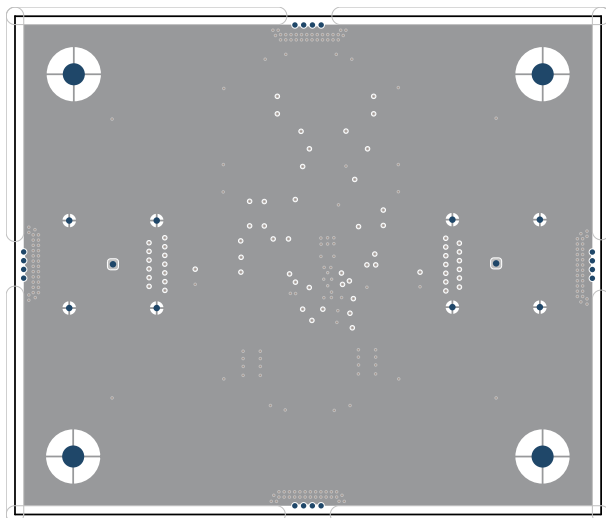
Figure 8-21. Mid Layer 1 Routing
