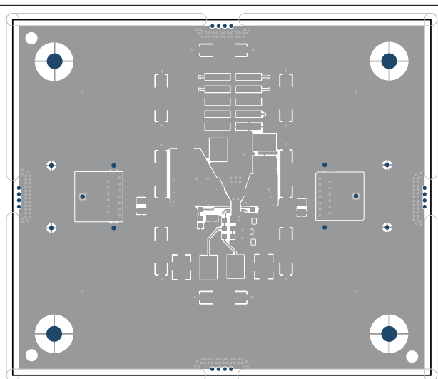
Figure 8-20. Top Layer Routing
