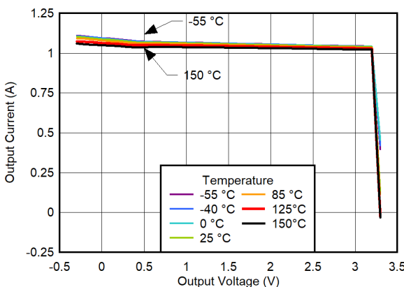
Figure 6-89. 80% Current Limit vs Temperature for V_{OUT} = 3.3\text{ V}
