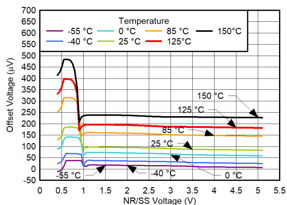
Figure 6-52. V_{OS} vs V_{NR/SS} and Temperature
