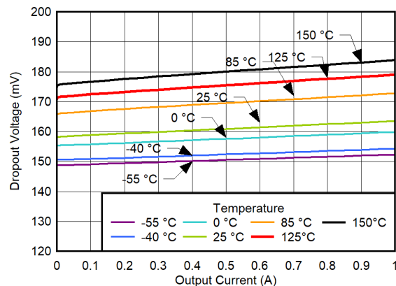
Figure 6-42. Dropout Voltage vs I_{OUT} for V_{OUT} = 1.8\text{ V}
