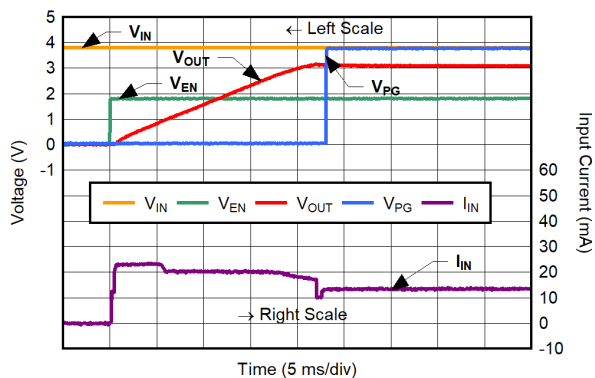
Figure 6-38. Inrush Current for C_{NR/SS} = 2.2\text{ }\mu\text{F}
