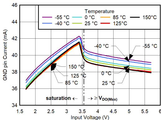
Figure 6-77. GND Pin Current vs V_{IN} and Temperature for I_{OUT} = 500\text{ mA}
