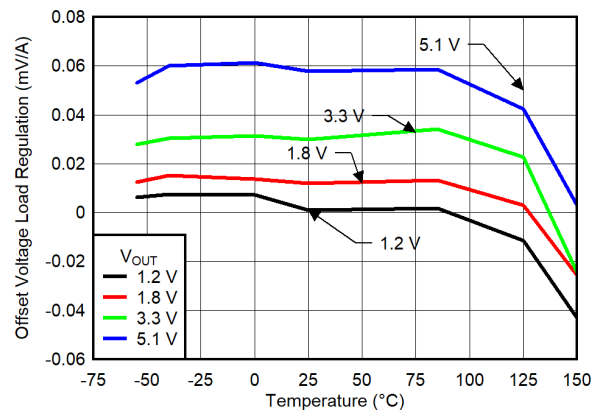
Figure 6-48. V_{OS} Load Regulation
