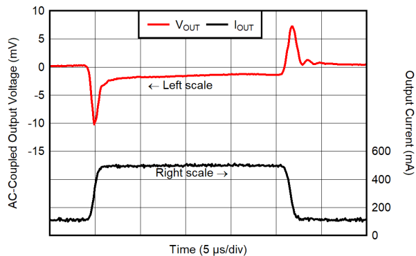
Figure 6-25. Load Transient Response for V_{OUT} = 3.3\text{ V} , I_{OUT} = 100\text{ mA} to 500\text{ mA}
