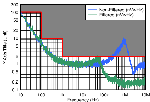
Figure 8-32. Noise vs Frequency
