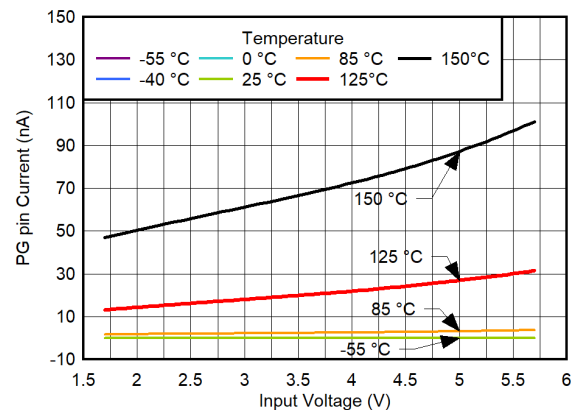
Figure 6-100. FB\_PG Pin Current vs V_{IN} and Temperature
