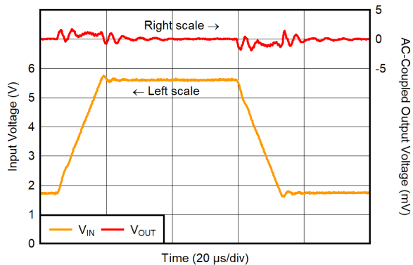
Figure 6-29. Line Transient Response for V_{OUT} = 1.2\text{ V} , I_{OUT} = 500\text{ mA}
