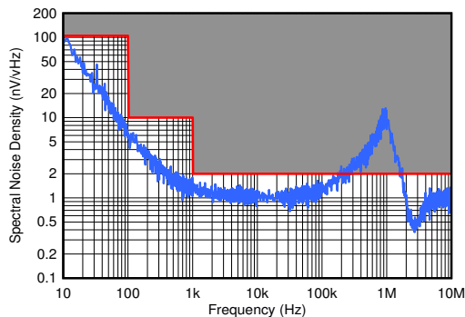
Figure 8-30. Output Noise vs Frequency
