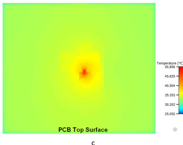
Figure 8-25. TPS7A94EVM-046 PCB Thermal Gradient
