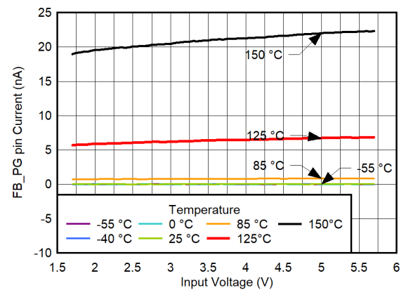
Figure 6-100. FB\_PG Pin Current vs V_{IN} and Temperature
