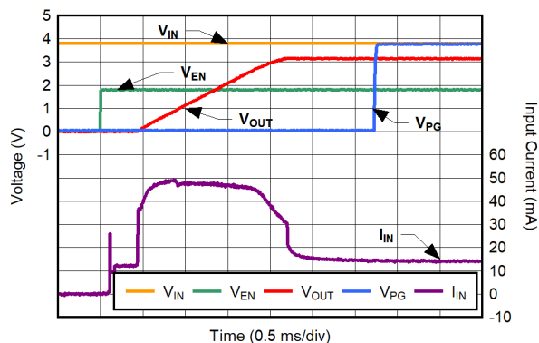
Figure 6-37. Inrush Current for C_{NR/SS} = 1.0\text{ }\mu\text{F}
