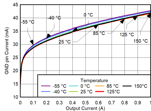
Figure 6-74. GND Pin Current vs I_{OUT} and Temperature for V_{OUT} = 5.1\text{ V}
