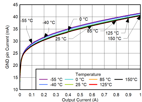
Figure 6-72. GND Pin Current vs I_{OUT} and Temperature for V_{OUT} = 1.2\text{ V}
