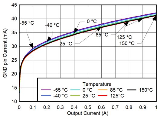
Figure 6-73. GND Pin Current vs I_{OUT} and Temperature for V_{OUT} = 3.3\text{ V}
