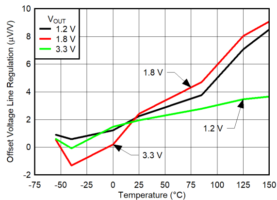
Figure 6-50. V_{OS} Line Regulation
