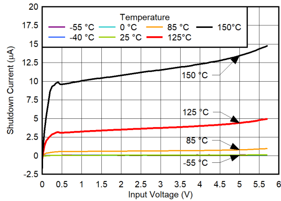
Figure 6-105. Shutdown Current vs V_{IN} and Temperature
