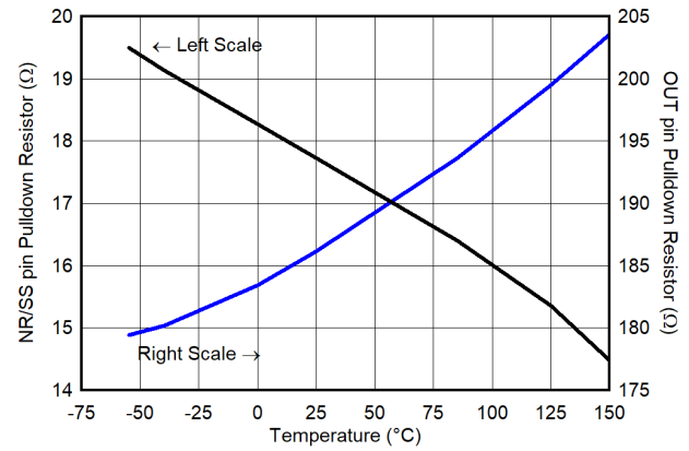
Figure 6-104. NR/SS and OUT Pulldown Resistors vs Temperature
