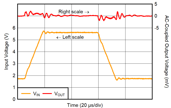
Figure 6-30. Line Transient Response for V_{OUT} = 1.2\text{ V} , I_{OUT} = 1\text{ A}
