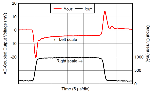
Figure 6-26. Load Transient Response for V_{OUT} = 3.3\text{ V} , I_{OUT} = 100\text{ mA} to 1\text{ A}
