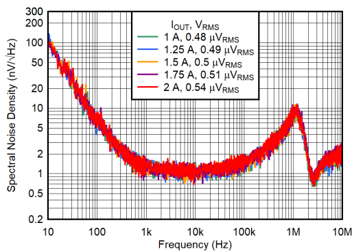
Figure 6-14. Output Voltage Noise Density vs Frequency for I_{OUT} and V_{OUT} = 3.3\text{ V}
