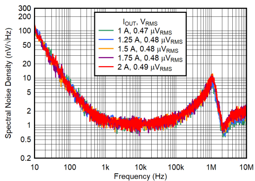
Figure 6-13. Output Voltage Noise Density vs Frequency for I_{OUT} and V_{OUT} = 1.8\text{ V}
