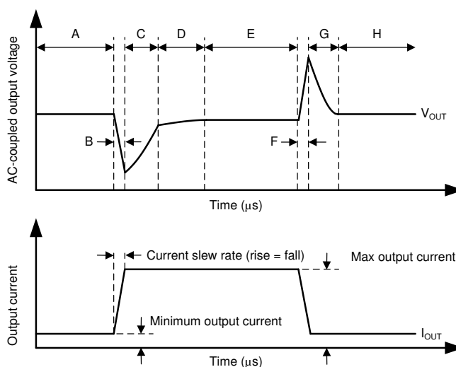
Figure 8-17. Load Transient Waveform
