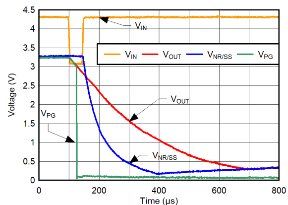
Figure 8-4. Example: Brownout
