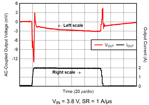
Figure 6-20. Load Transient Response for V_{OUT} = 3.3\text{ V} , I_{OUT} = 100\text{ mA} to 2\text{ A}
