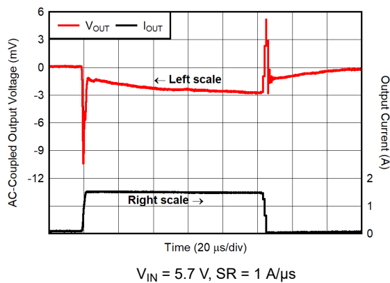
Figure 6-21. Load Transient Response for V_{OUT} = 5.2\text{ V} , I_{OUT} = 100\text{ mA} to 1.5\text{ A}
