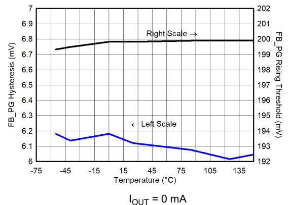
Figure 6-66. V_{FB\_PG} Hysteresis and Threshold vs Temperature
