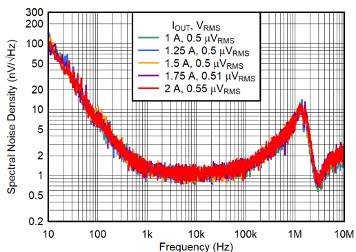
Figure 6-15. Output Voltage Noise Density vs Frequency for I_{OUT} and V_{OUT} = 5.0\text{ V}
