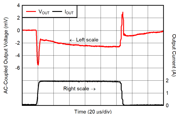
Figure 6-18. Load Transient Response for V_{OUT} = 1.2\text{ V} , I_{OUT} = 100\text{ mA} to 2\text{ A}
