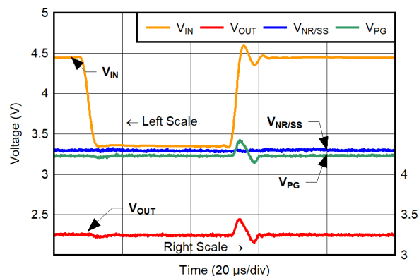
Figure 8-5. Example: Brownout With Overshoot Recovery
