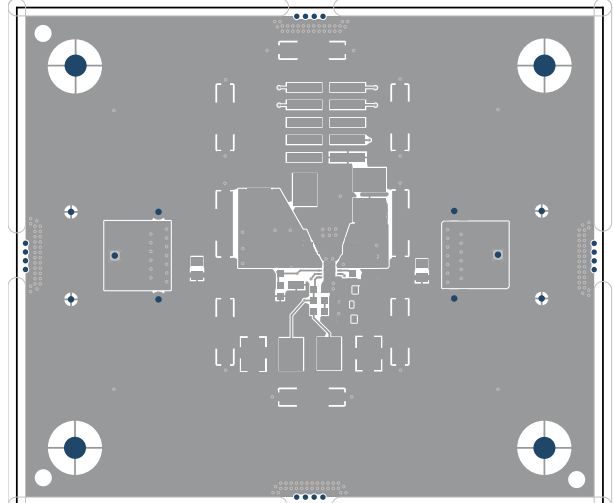
Figure 8-19. Top Layer Routing
