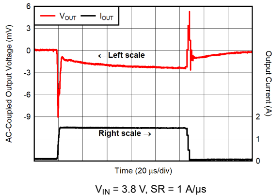
Figure 6-19. Load Transient Response for V_{OUT} = 3.3\text{ V} , I_{OUT} = 100\text{ mA} to 1.5\text{ A}
