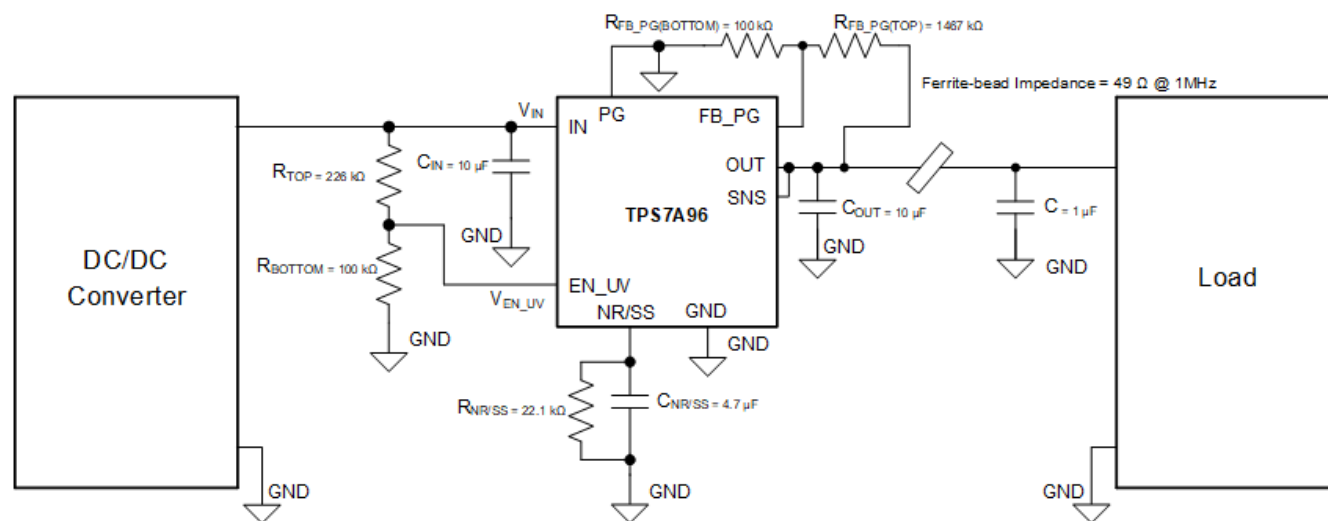
Figure 8-27. Typical Application Circuit With Added Pi-Filter
