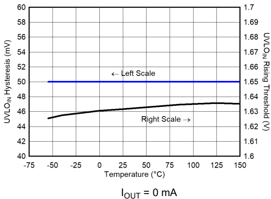
Figure 6-63. UVLO_{IN} vs Temperature
