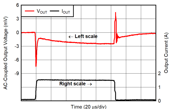
Figure 6-17. Load Transient Response for V_{OUT} = 1.2\text{ V} , I_{OUT} = 100\text{ mA} to 1.5\text{ A}
