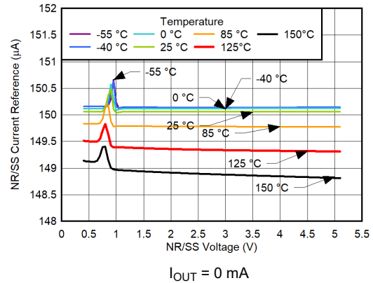
Figure 6-38. I_{NR/SS} vs V_{NR/SS} and Temperature
