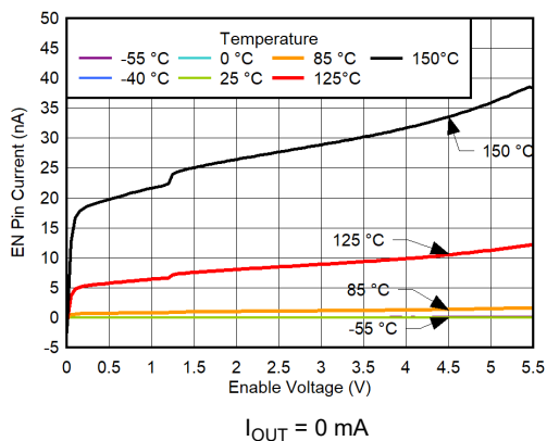
Figure 6-65. EN Pin Current vs V_{EN} and Temperature for V_{IN} = 5.7\text{ V}
