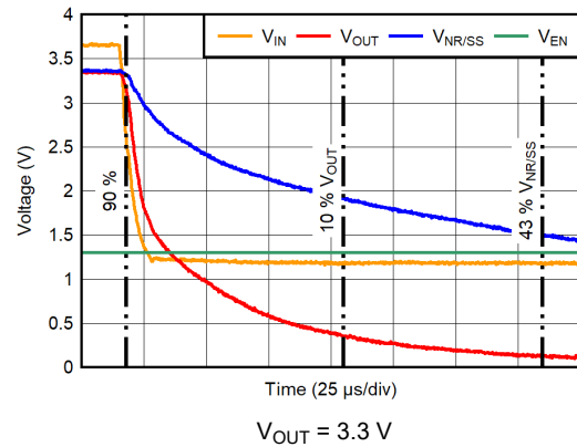
Figure 6-26. Shutdown Waveform for UVLO_{(IN)}
