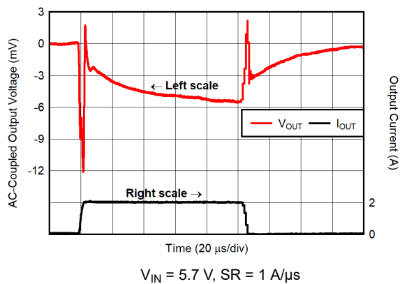
Figure 6-22. Load Transient Response for V_{OUT} = 5.2\text{ V} , I_{OUT} = 100\text{ mA} to 2\text{ A}
