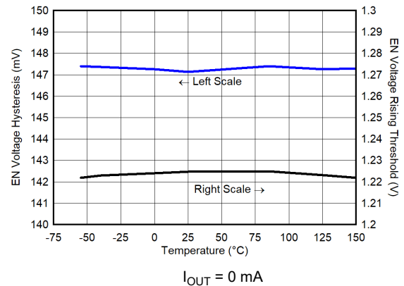
Figure 6-64. V_{EN} Hysteresis and Threshold vs Temperature
