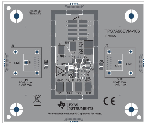
Figure 8-18. Top Composite View
