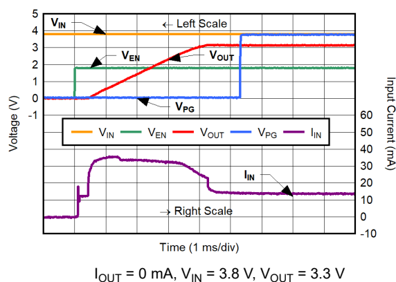
Figure 6-29. Inrush Current for C_{NR/SS} = 2.2\text{ }\mu\text{F}
