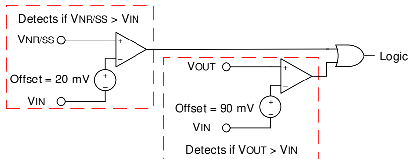
Figure 8-1. Overshoot Prevention Circuit
