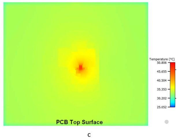
Figure 8-24. TPS7A96EVM-106 PCB Thermal Gradient
