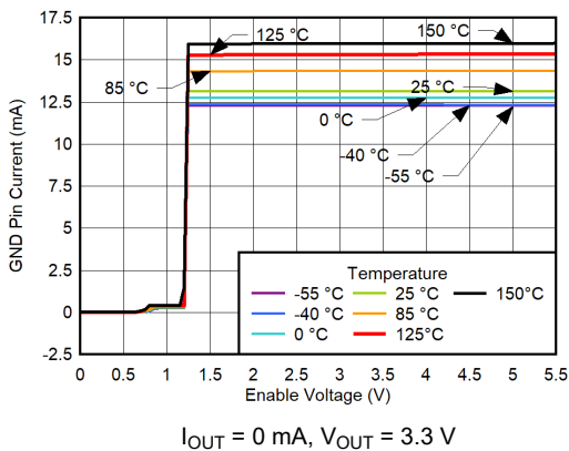
Figure 6-59. GND Pin Current vs V_{EN} and Temperature for V_{IN} = 5.7\text{ V}
