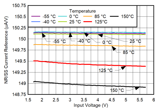
Figure 6-42. I_{NR/SS} vs V_{IN} and Temperature for V_{OUT} = 1.2\text{ V}
