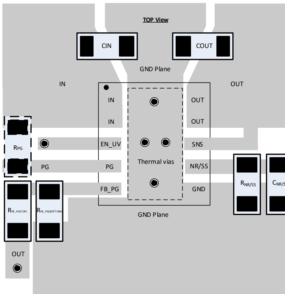
Figure 8-33. Example Layout
