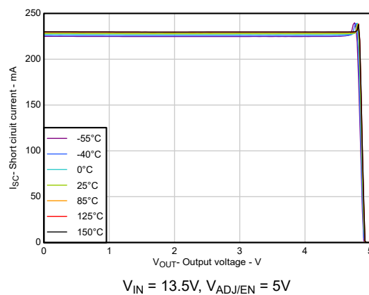
Figure 5-16. Current Limit vs Output Voltage
