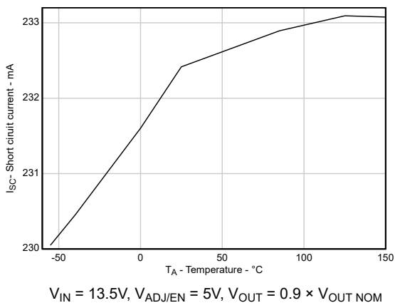
Figure 5-15. Current Limit vs Ambient Temperature
