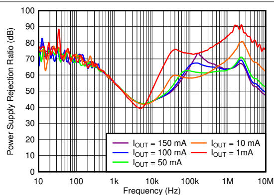
Figure 8-6. PSRR
