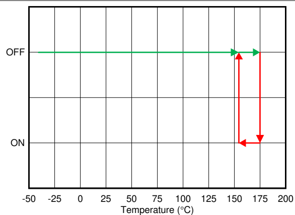
Figure 6-30. Thermal Shutdown
