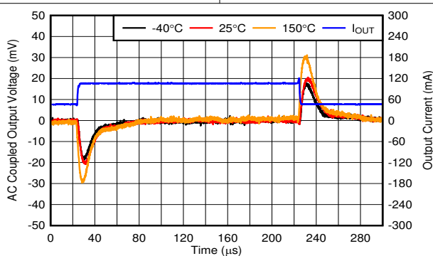
Figure 8-7. Transient Response
