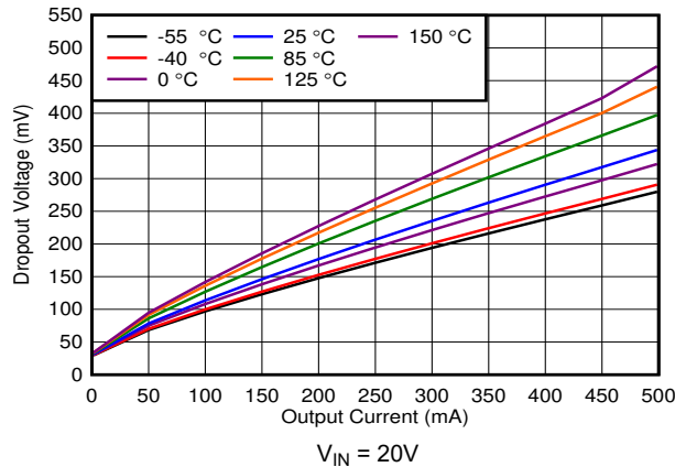
Figure 5-9. Dropout Voltage ( V_{DO} ) vs I_{OUT}
