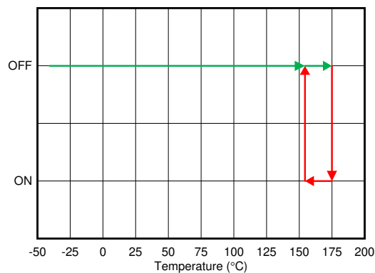
Figure 5-38. Thermal Shutdown
