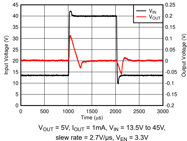
Figure 5-15. Line Transients
