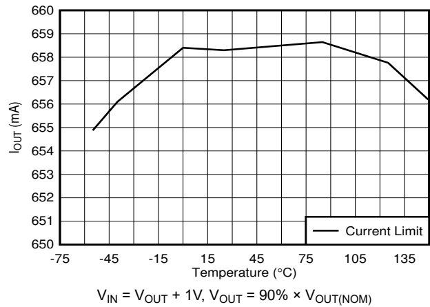
Figure 5-26. Output Current Limit vs Temperature
