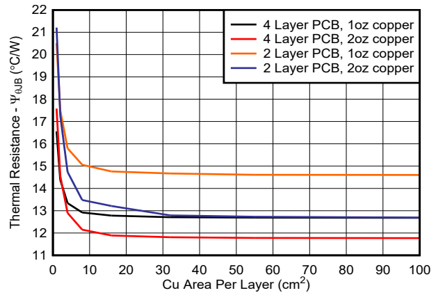
Figure 7-3. \psi_{JB} vs Copper Area (DDA Package)
