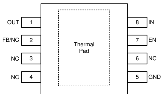
Figure 4-2. DDA Package (Without PG), 8-Pin HSOIC (Top View)
