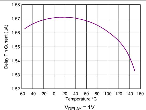
Figure 5-36. Delay Pin Current vs Temperature
