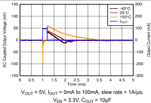
Figure 5-17. Load Transient, No Load to 100mA
