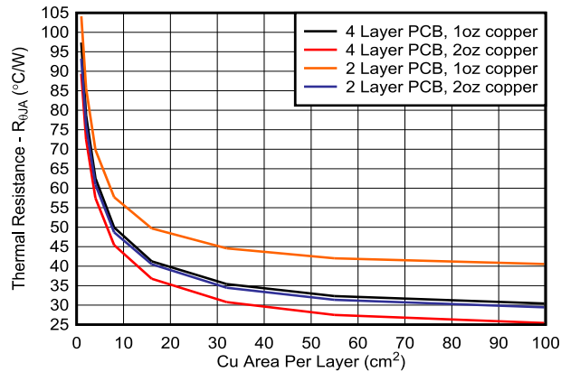
Figure 7-2. R_{\theta JA} vs Copper Area (DDA Package)
