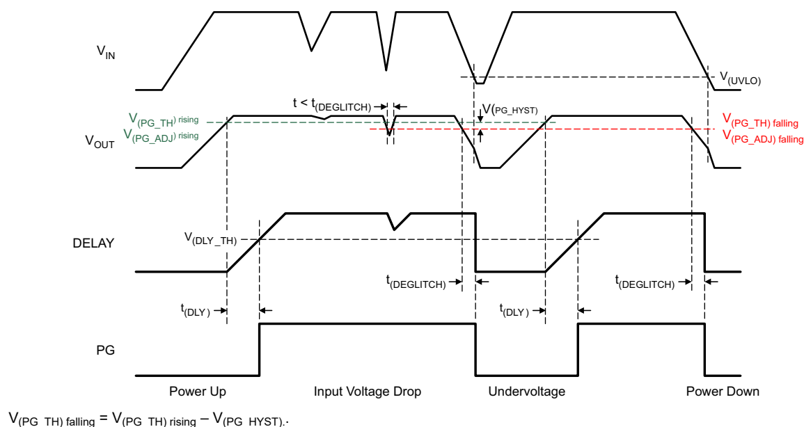
Figure 6-4. Typical Power-Good Timing Diagram
