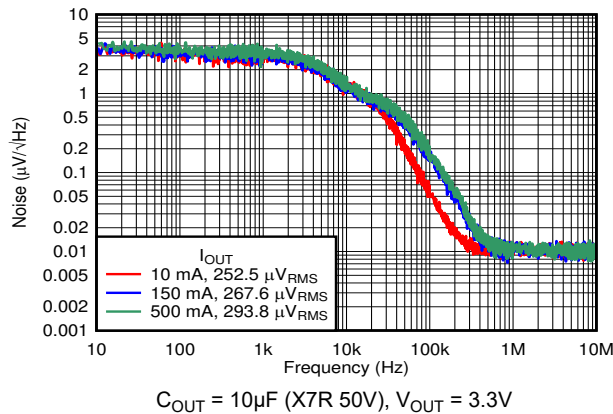
Figure 5-13. Noise vs Frequency
