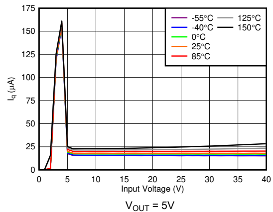
Figure 5-28. Quiescent Current ( I_Q ) vs V_{IN}
