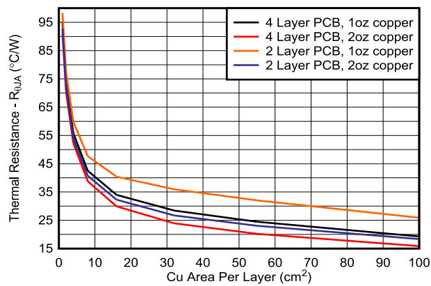
Figure 7-4. R_{\theta JA} vs Copper Area (KVU Package)
