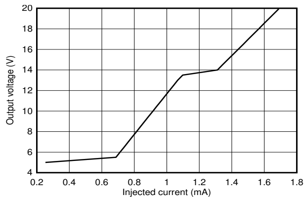
Figure 5-37. Output Voltage vs Injected Current
