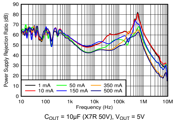
Figure 5-11. PSRR vs Frequency and I_{OUT}
