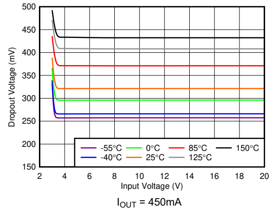
Figure 5-10. Dropout Voltage ( V_{DO} ) vs V_{IN}
