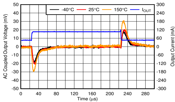
Figure 5-19. Load Transient, 45mA to 105mA
