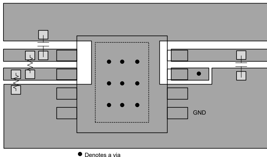
Figure 7-11. DDA Package Adjustable Output
