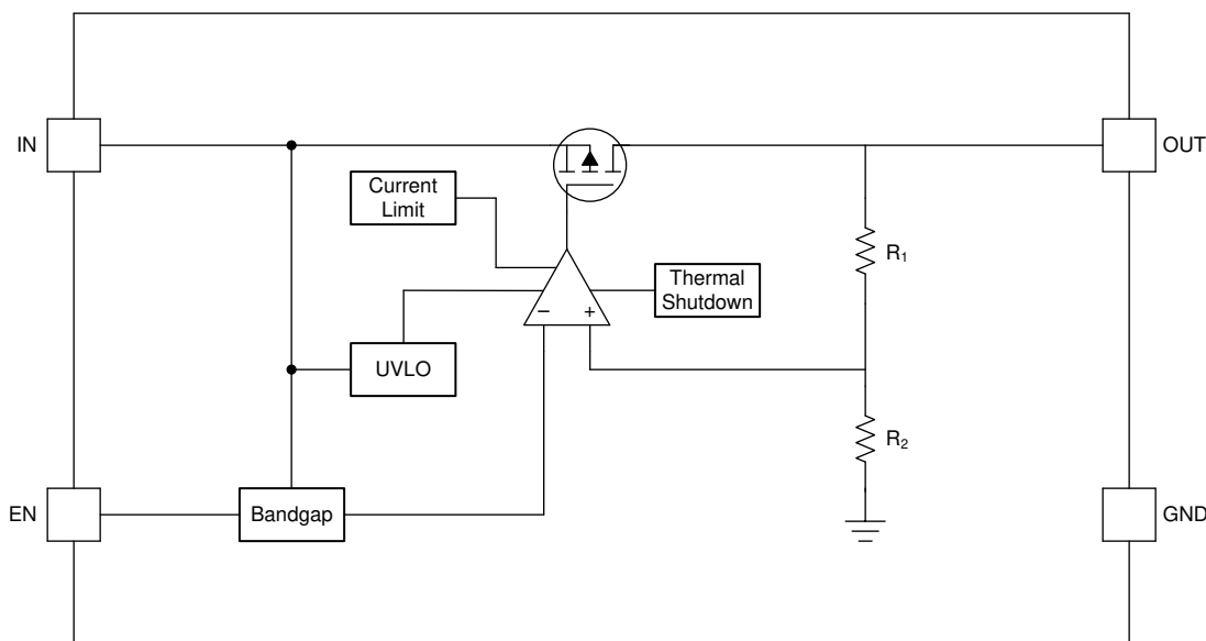
Figure 6-1. TPS7B86-Q1 Fixed Output Without PG
