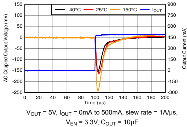
Figure 5-25. Load Transient, No Load to 500mA Rising Edge
