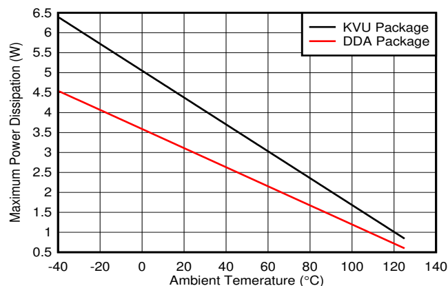
Figure 7-6. TPS7B86-Q1 Allowable Power Dissipation
