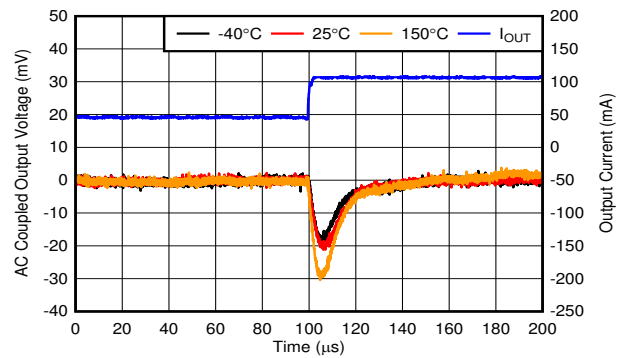
Figure 5-20. Load Transient, 45mA to 105mA Rising Edge
