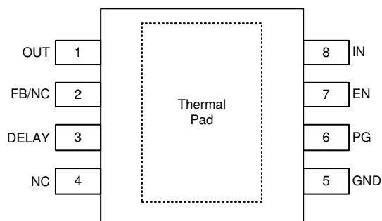
Figure 4-3. DDA Package (With PG), 8-Pin HSOIC, B Version (Top View)
