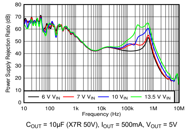
Figure 5-14. PSRR vs Frequency and V_{IN}
