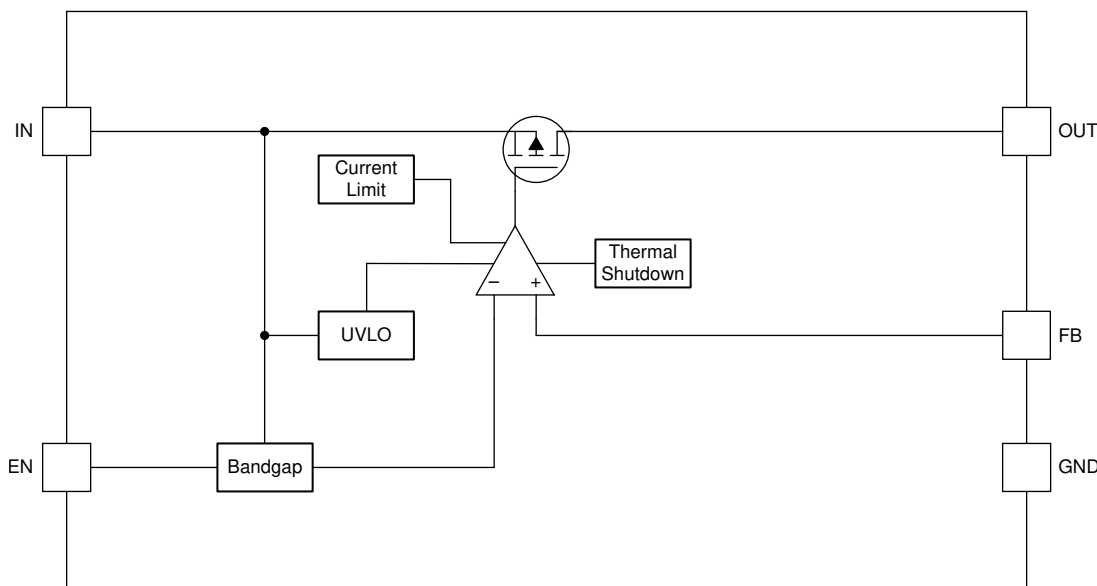
Figure 6-2. TPS7B86-Q1 Adjustable Output Without PG
