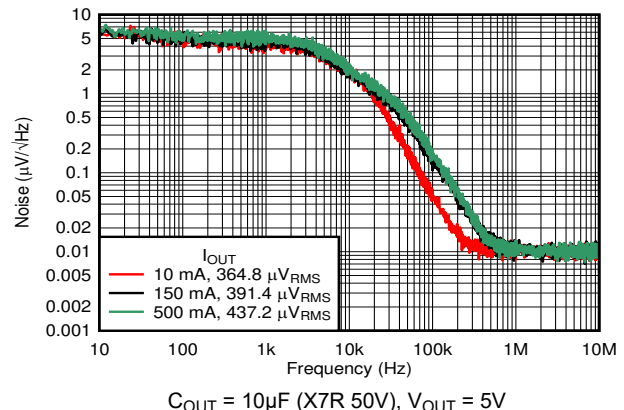
Figure 5-12. Noise vs Frequency
