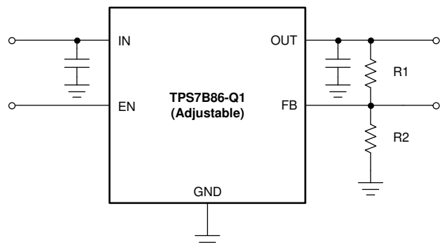
Adjustable Output Voltage
