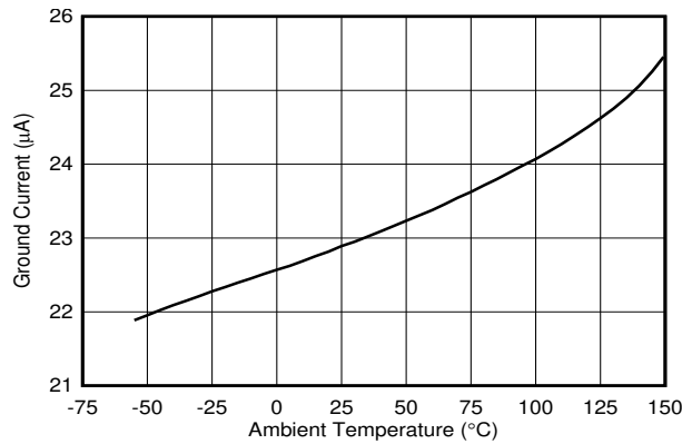
Figure 5-31. Ground Current at 500µA
