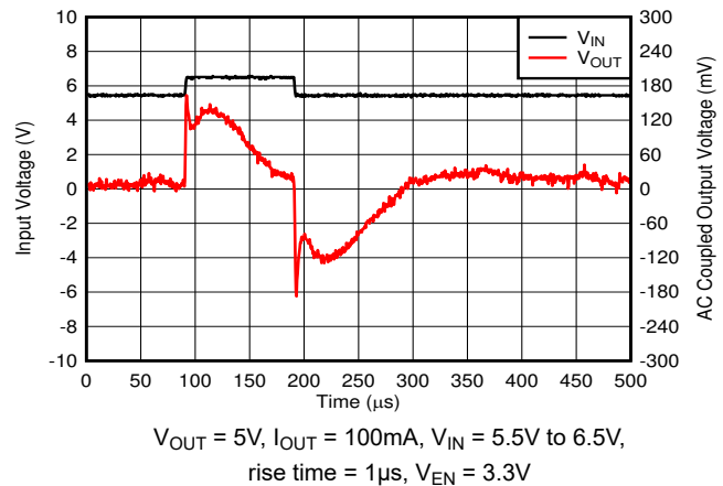
Figure 5-16. Line Transients
