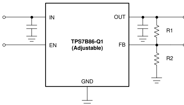
Figure 7-7. Typical Application Schematic for the TPS7B86-Q1
