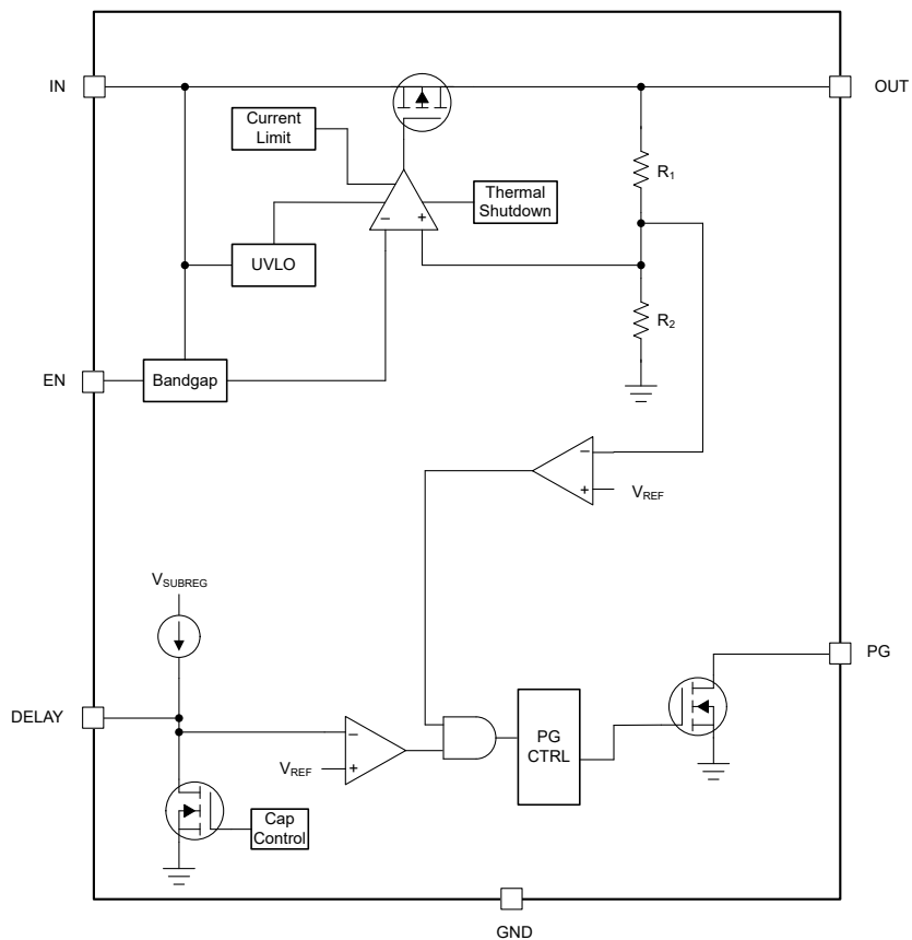
Figure 6-3. TPS7B86-Q1 With PG
