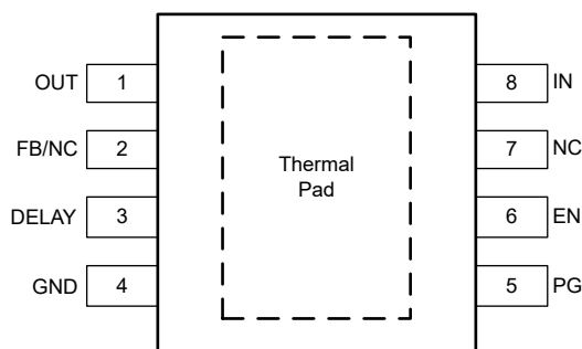
Figure 4-4. DDA Package (With PG), 8-Pin HSOIC, D Version (Top View)
