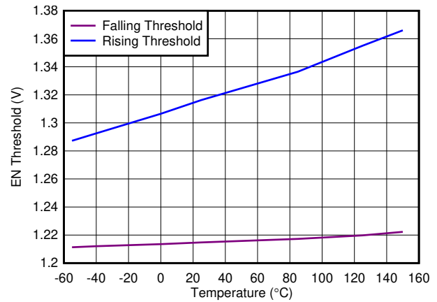
Figure 5-32. EN Threshold vs Temperature
