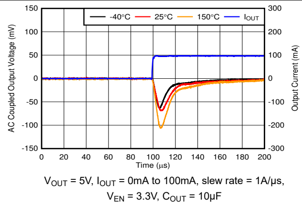
Figure 5-18. Load Transient, No Load to 100mA Rising Edge
