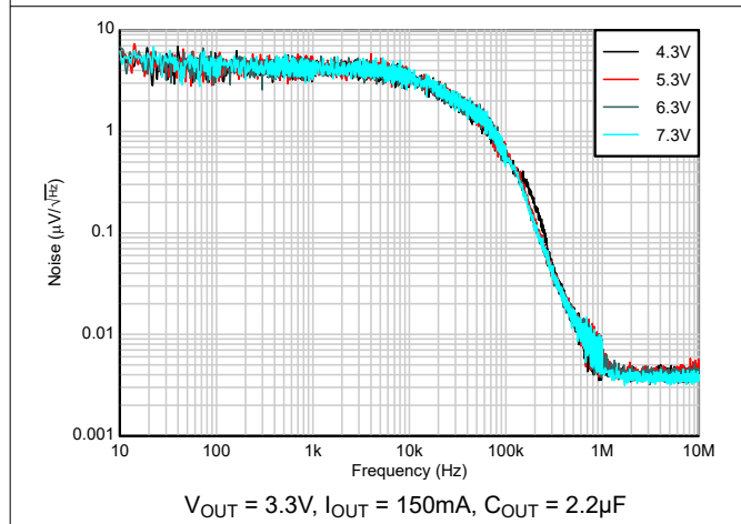
Figure 5-27. Noise vs V_{IN}
