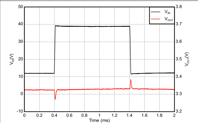
V_{IN} = 12\text{V} to 40\text{V} , V_{OUT} = 3.3\text{V} , I_{OUT} = 150\text{mA} , dV_{IN}/dt = 2\text{V}/\mu\text{s}
