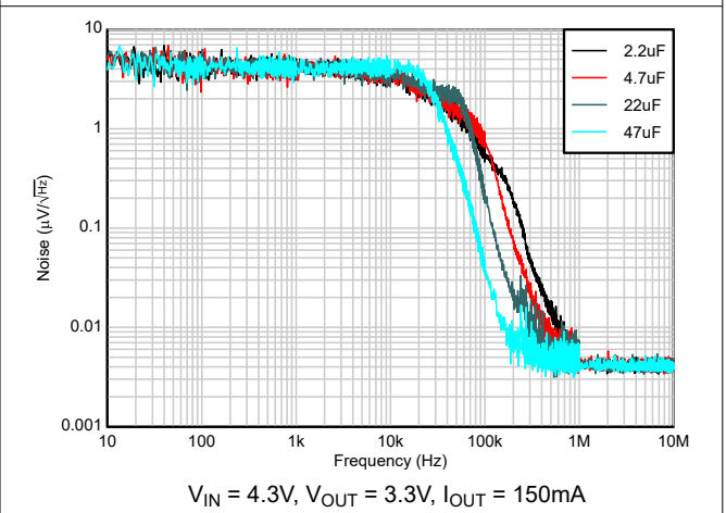
Figure 5-28. Noise vs C_{OUT}
