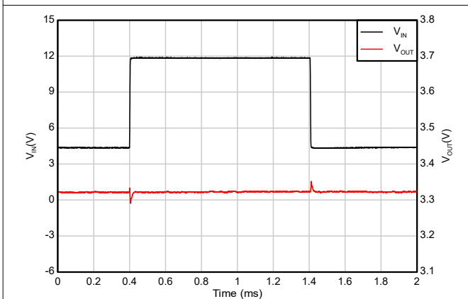
V_{IN} = 4.3\text{V} to 12\text{V} , V_{OUT} = 3.3\text{V} , I_{OUT} = 150\text{mA} , dV_{IN}/dt = 2\text{V}/\mu\text{s}
