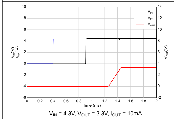
Figure 5-39. Start-up with sequencing ( V_{IN} after EN)
