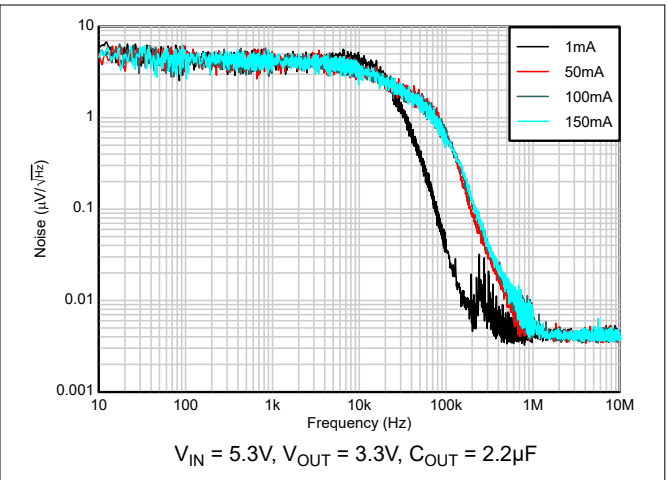
Figure 5-26. Noise vs I_{OUT}
