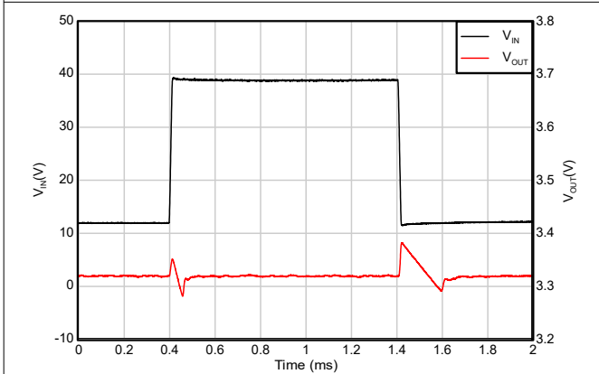
V_{IN} = 12\text{V} to 40\text{V} , V_{OUT} = 3.3\text{V} , I_{OUT} = 1\text{mA} , dV_{IN}/dt = 2\text{V}/\mu\text{s}
