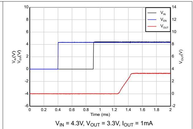
Figure 5-38. Start-up with sequencing ( V_{IN} after EN)
