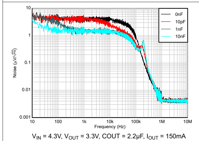
Figure 5-29. Noise vs C_{FF}
