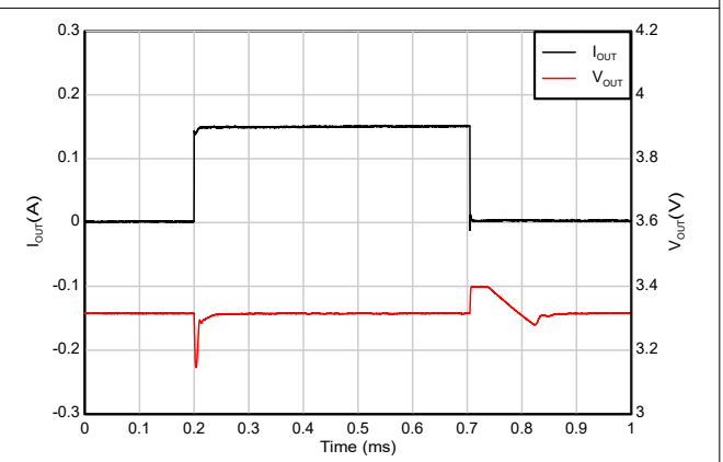
V_{IN} = 4.3\text{V} , V_{OUT} = 3.3\text{V} , I_{OUT} = 0\text{mA} to 150\text{mA} , dI_{OUT}/dt = 2\text{A}/\mu\text{s}
