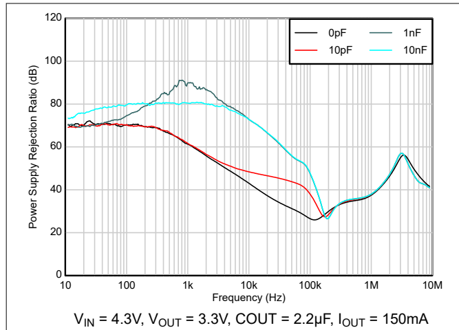
Figure 5-25. PSRR vs C_{FF}
