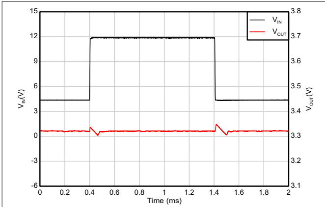
V_{IN} = 4.3\text{V} to 12\text{V} , V_{OUT} = 3.3\text{V} , I_{OUT} = 1\text{mA} , dV_{IN}/dt = 2\text{V}/\mu\text{s}
