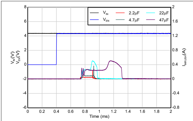
V_{IN} = 4.3\text{V} , V_{OUT} = 3.3\text{V} , I_{OUT} = 0\text{mA}
