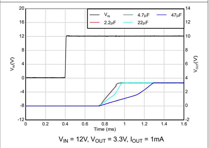
Figure 5-30. Start-up vs C_{OUT}
