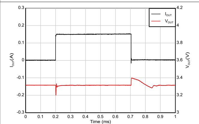
V_{IN} = 4.3\text{V} , V_{OUT} = 3.3\text{V} , I_{OUT} = 1\text{mA} to 150\text{mA} , dI_{OUT}/dt = 2\text{A}/\mu\text{s}
