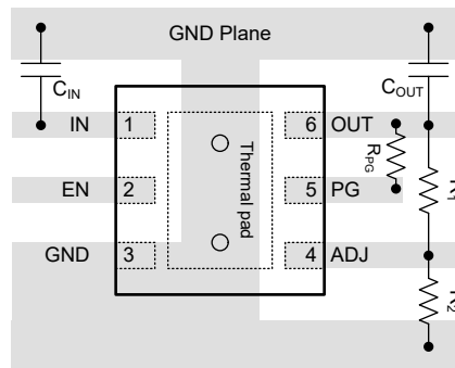
Figure 7-17. Example Layout for TPS7E66-Q1 DRV Package
