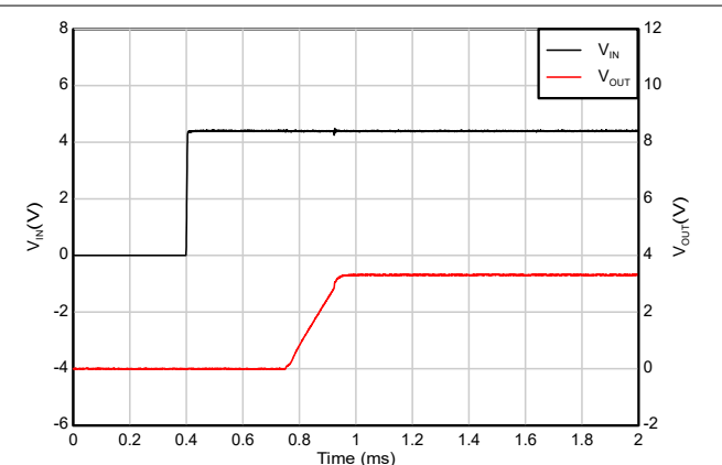
Figure 7-8. Start-up with EN & V_{IN} tied together
