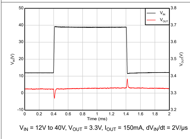
Figure 5-43. Line Transient (12V to 40V)
