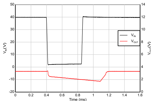
Figure 5-39. Dropout Recovery
