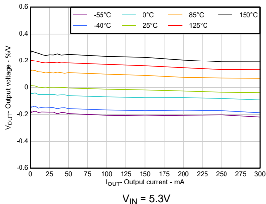
Figure 5-5. Accuracy vs Output Current
