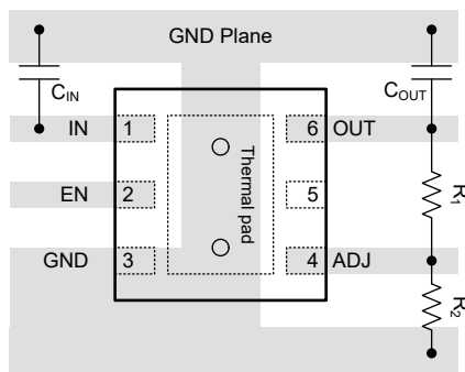
Figure 7-12. Example Layout for TPS7E82 DRV Package
