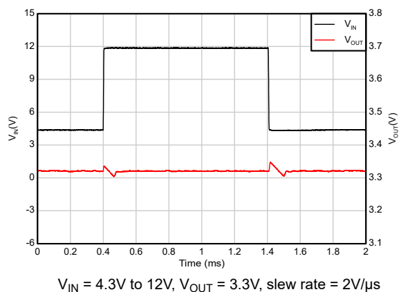
Figure 5-29. Line Transient
