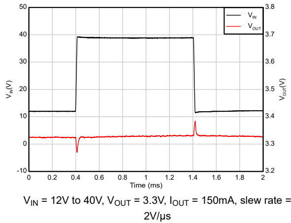
Figure 7-6. Line Transient
