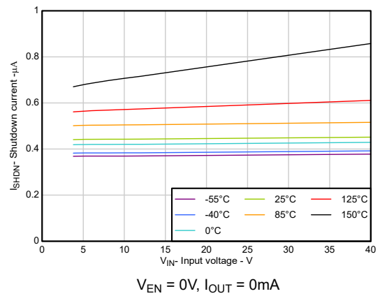
Figure 5-14. Shutdown Current vs Input Voltage
