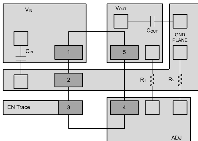
Figure 7-11. Example Layout for TPS7E82 DBV Package
