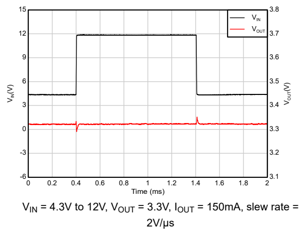
Figure 5-30. Line Transient
