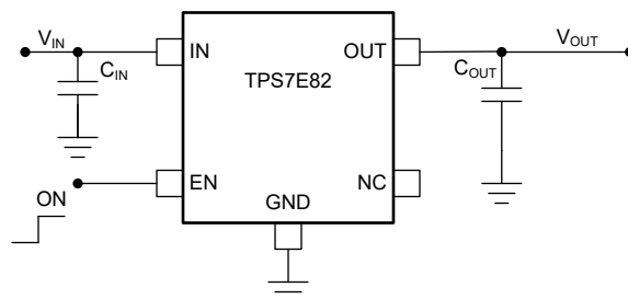
Figure 7-4. TPS7E82 Typical Application Circuit (Fixed-Voltage Version)
