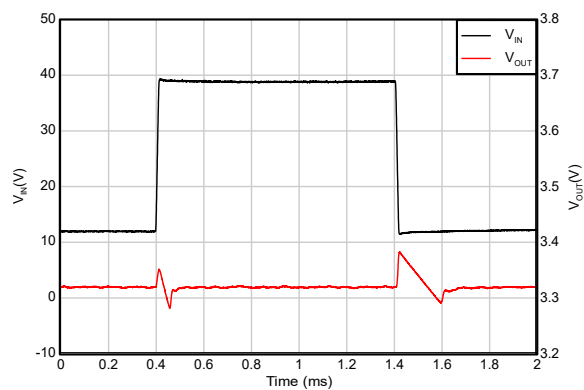
Figure 5-31. Line Transient
