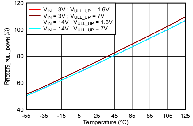
Figure 6-34. RESET1 Pull-Down Resistance vs Temperature Across V_{PULL\_UP} and V_{IN} at I_{LOAD} = 2mA for the TPS7H3124
