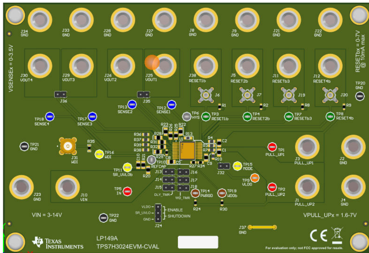
Figure 9-7. Printed Circuit Board Layout Example: Top Layer 3D View
