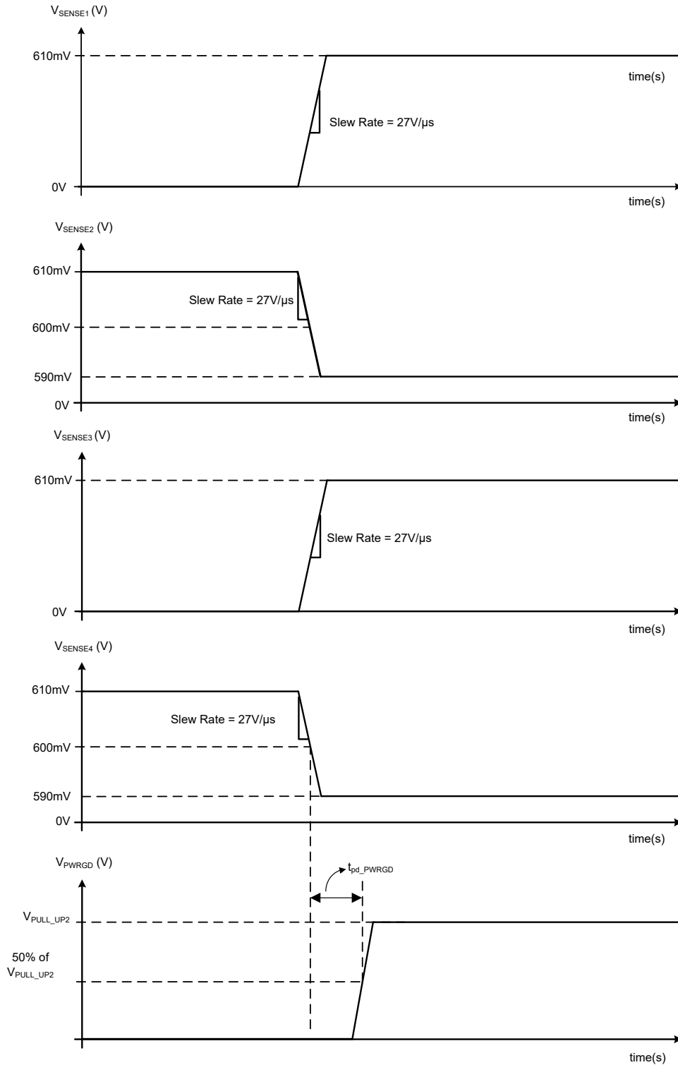
Figure 7-4. PWRGD Propagation Delay ( t_{\text{pd\_PWRGD}} ) for TPS7H3024 (Push-Pull)
