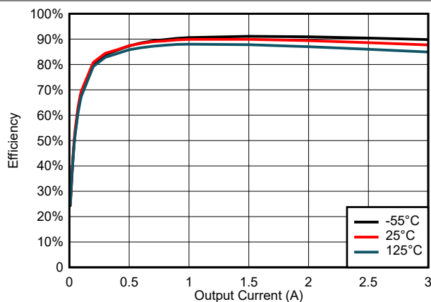
Figure 6-49. Efficiency fo V_{\text{IN}} = 5.5\ \text{V}
