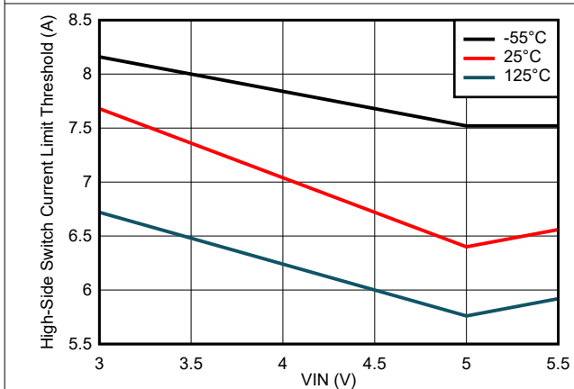
Figure 6-11. High-Side Switch Current Limit Threshold Variation
