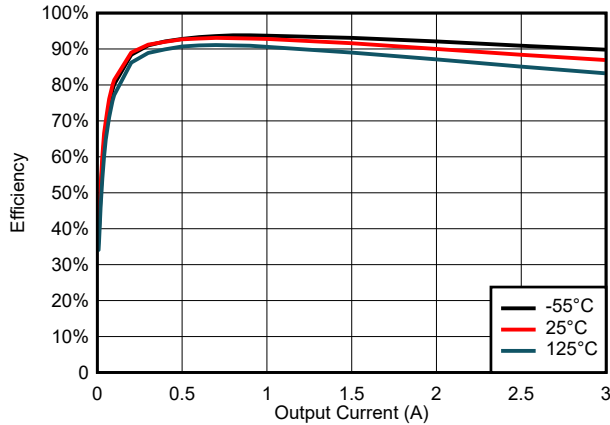
Figure 6-31. Efficiency for V_{\text{IN}} = 5 \text{ V}
