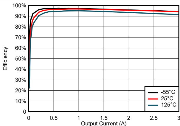
Figure 6-33. Efficiency for V_{\text{IN}} = 5 \text{ V}
