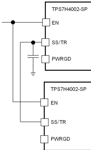
Figure 7-6. Ratiometric Start-Up Sequence
