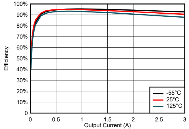
Figure 6-32. Efficiency for V_{\text{IN}} = 5 \text{ V}
