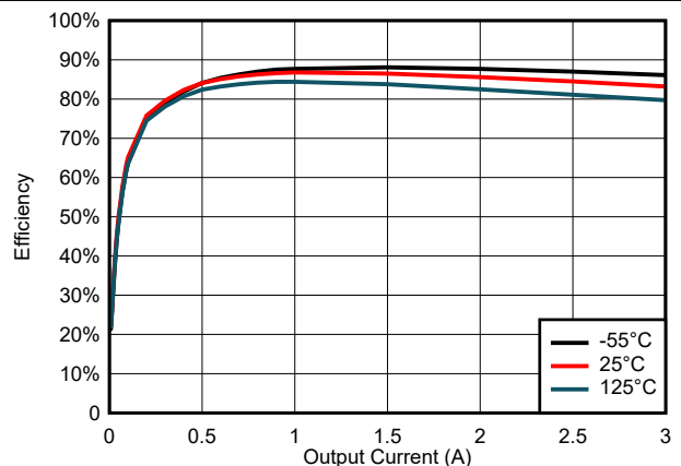
Figure 6-34. Efficiency for V_{\text{IN}} = 5 \text{ V}
