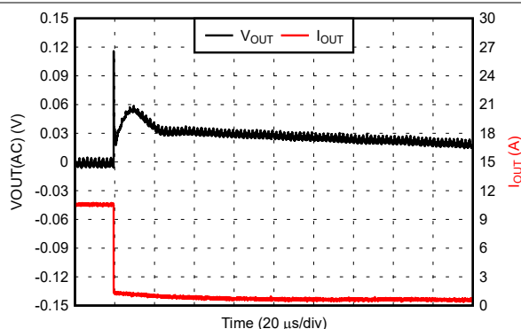
Figure 7-66. Load Step: 10.6A to 0.6A
