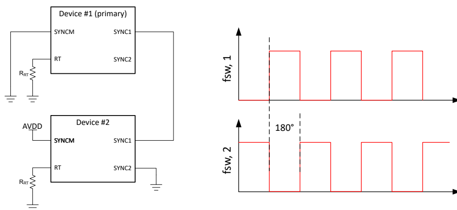
Figure 9-13. Parallel Operation With Two Devices
