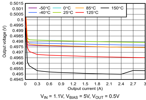
Figure 5-19. Load Regulation
