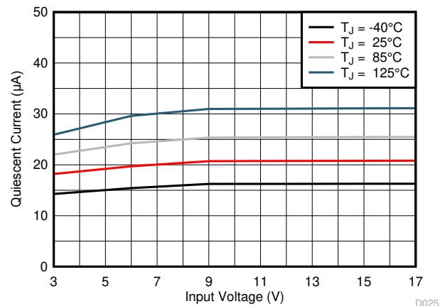
Figure 6-2. Quiescent Current
