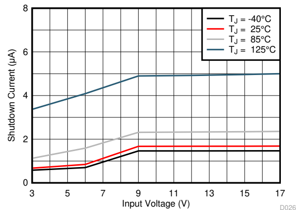
Figure 6-3. Shutdown Current
