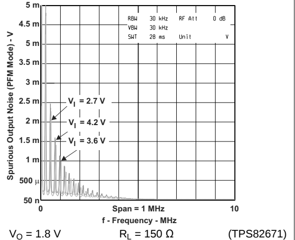
Figure 4. Spurious Output Noise (PFM Mode) vs. Frequency
