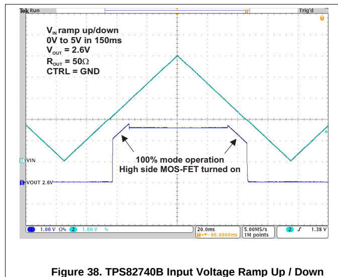
Figure 38. TPS82740B Input Voltage Ramp Up / Down
