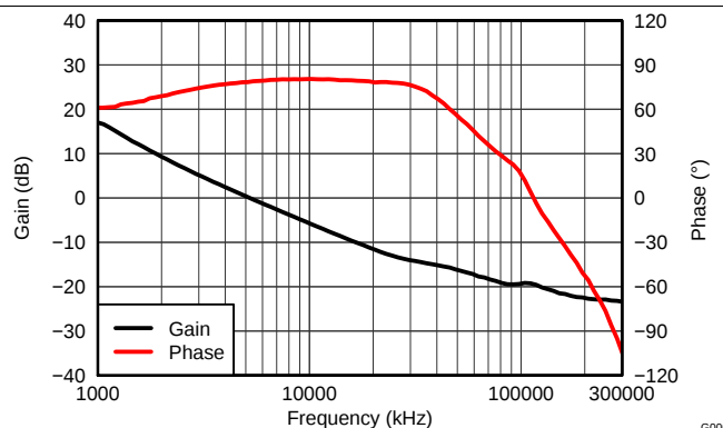
Figure 26. V_{IN}=5\text{ V} , V_{OUT}=-12\text{ V} , I_{OUT}=0.3\text{ A} , C_{OUT}=4 \times 22\mu\text{F} ceramic, f_{SW}=800\text{ kHz}
