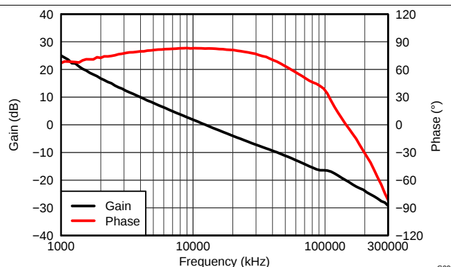
Figure 30. V_{IN}=24\text{ V} , V_{OUT}=-12\text{ V} , I_{OUT}=1.5\text{ A} , C_{OUT}=4 \times 22\mu\text{F} ceramic, f_{SW}=800\text{ kHz}
