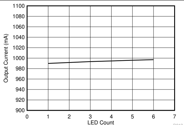
Figure 6-3. Output Current vs LED Count
