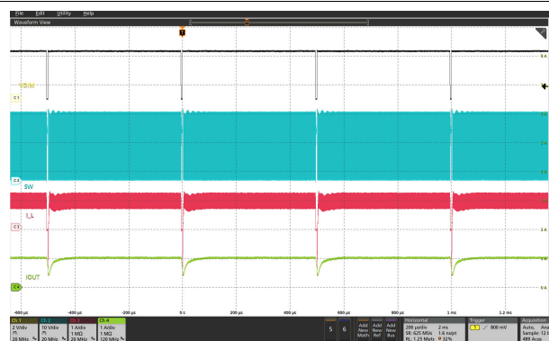
Figure 8-25. LED PWM Dimming at 99% Duty Cycle and 2 kHz
