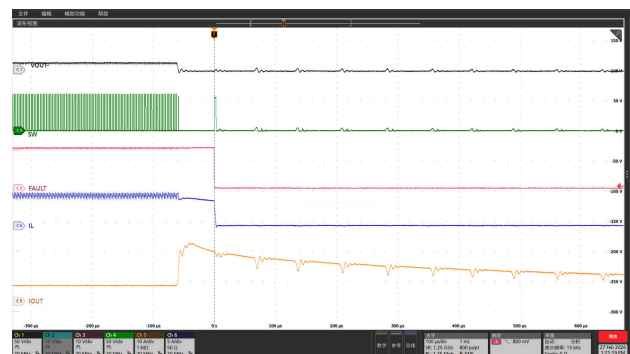
Figure 7-7. Shutdown at ADIM = 0V
