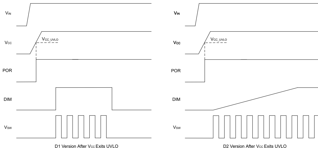
Figure 7-2. Startup Sequence
