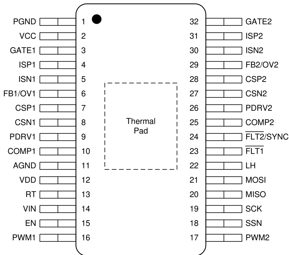
Figure 5-2. DAP Package 32-Pin TSSOP with PowerPAD Top View
