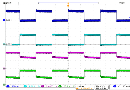
CH1: Boost I_{LED} CH2: Buck-Boost I_{LED} current CH3: Boost LED+ voltage (12xLED) CH4: Buck-Boost LED+ voltage (3xLED)
