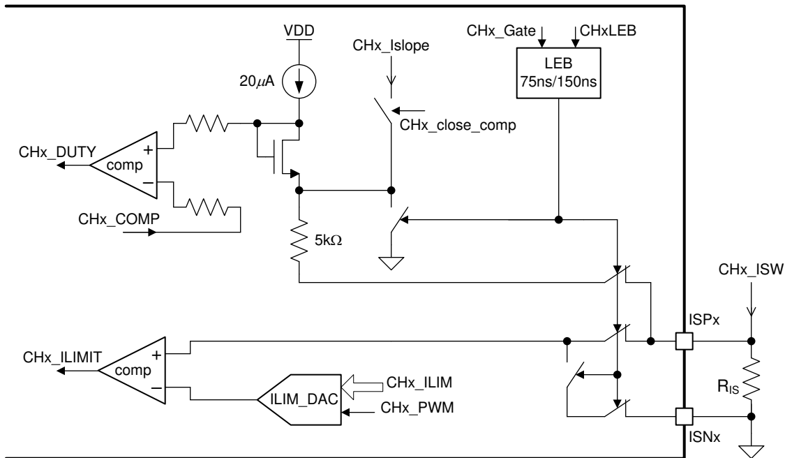
7.3.9 Slope Compensation
