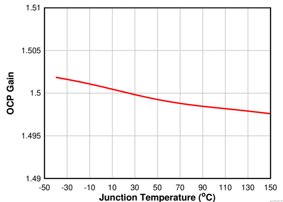
Figure 6-21. Over Current Protection Gain vs Junction Temperature
