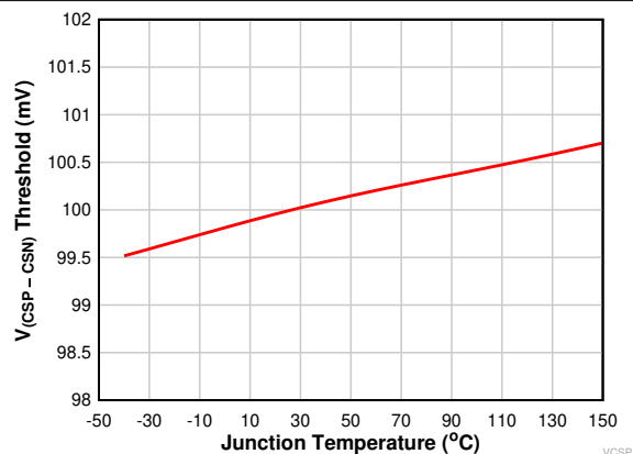
Figure 6-20. V_{(CSP - VCSN)} Voltage vs Junction Temperature
