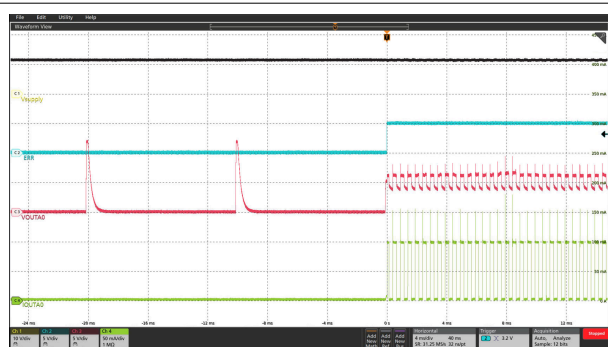
Figure 5-27. Single-LED Short-Circuit Detection in Normal Mode
