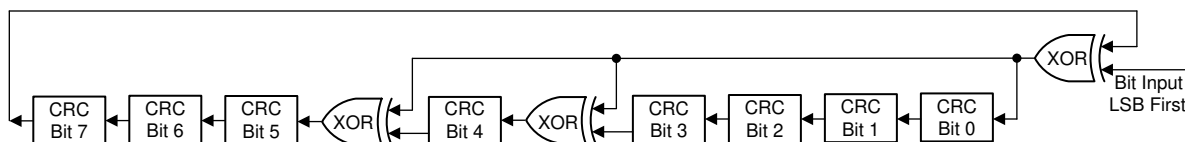
Figure 6-7. CRC Algorithm Diagram
