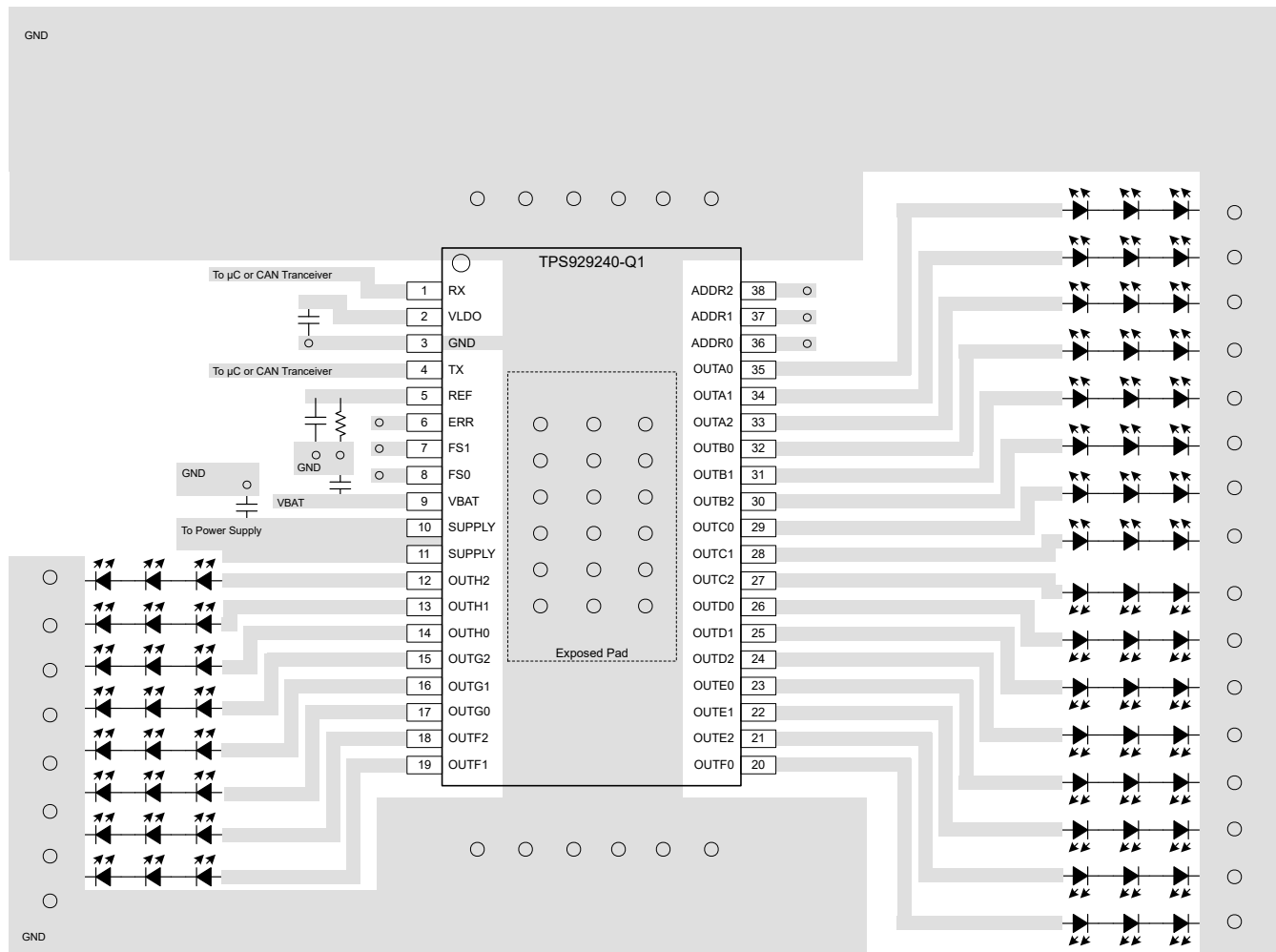
Figure 7-5. TPS929240-Q1 Layout
