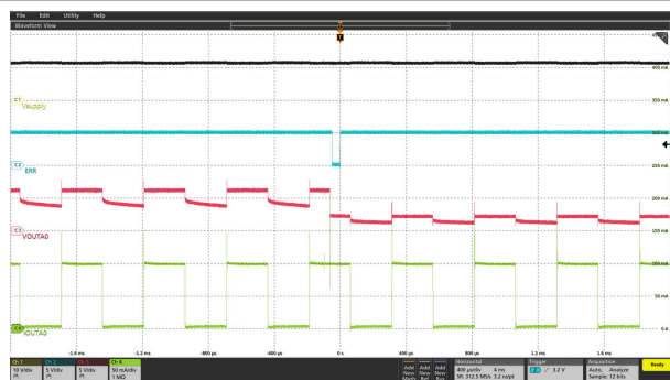
Figure 5-25. LED Open-Circuit Detection in Normal Mode
