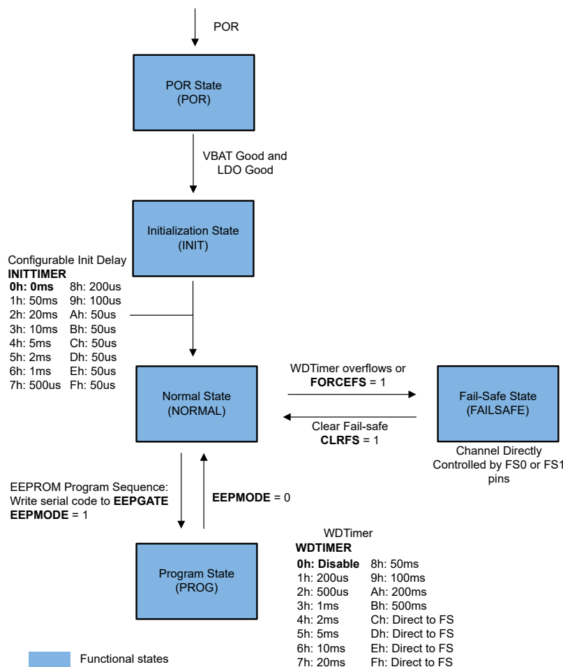
Figure 6-9. Device Functional Mode Statemachine
