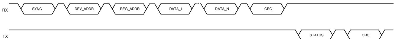
Figure 6-16. Multiple Data Bytes Write in Burst Mode
