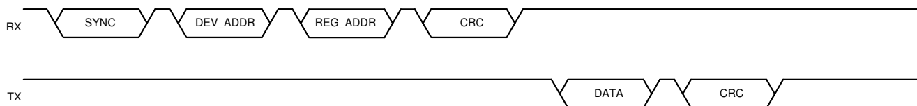
Figure 6-12. Single-Byte Readback Command
