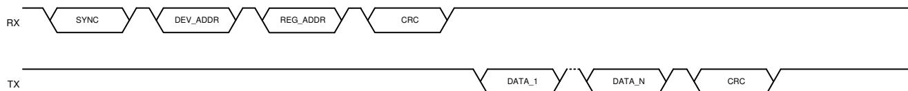
Figure 6-17. Multiple Data Bytes Read in Burst Mode
