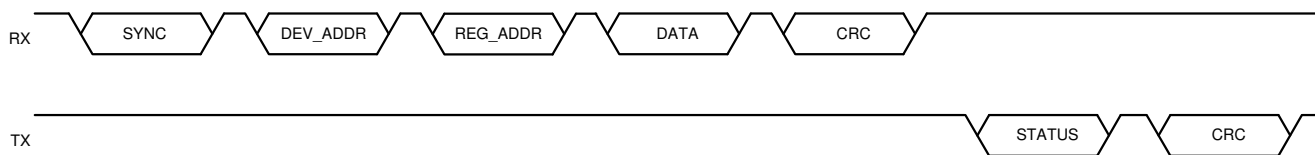
Figure 6-11. Single-Byte Write Command with Status Feedback
