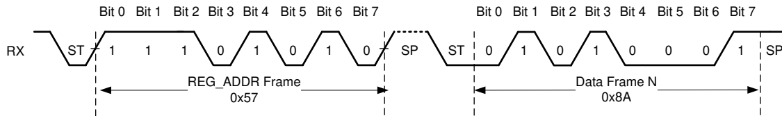
Figure 6-14. Address and Data Bytes
