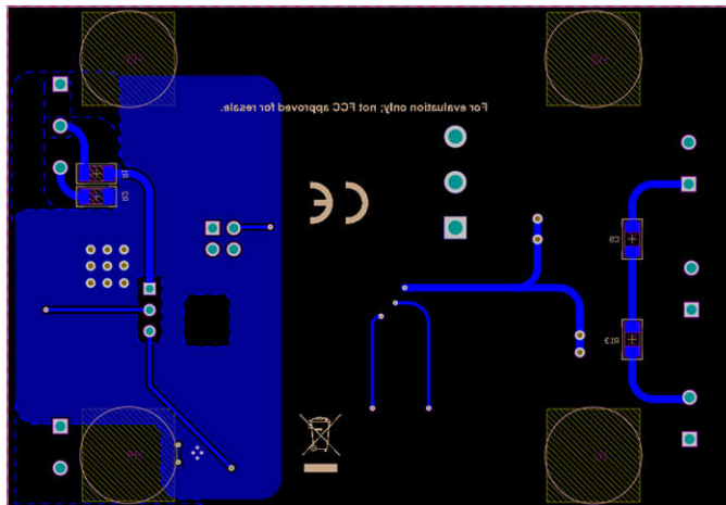
Figure 9-14. Bottom Layer
