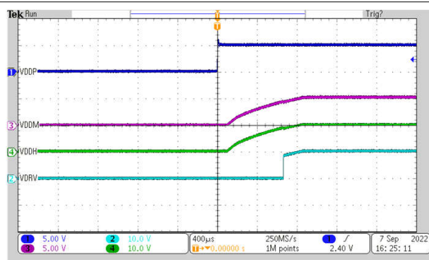
Figure 9-6. t_{LH\_VDRV} , Three-Wire Mode, TPSI3050
