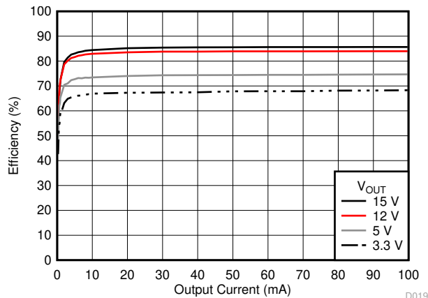
Figure 6-16. Efficiency
