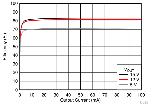
Figure 6-21. Efficiency
