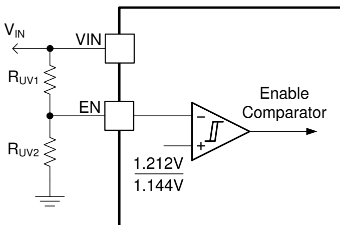
Figure 7-2. Programmable V_{IN} UVLO with Fixed Hysteresis
