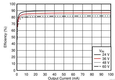
Typical Efficiency, V_{OUT} = 15\text{ V}
