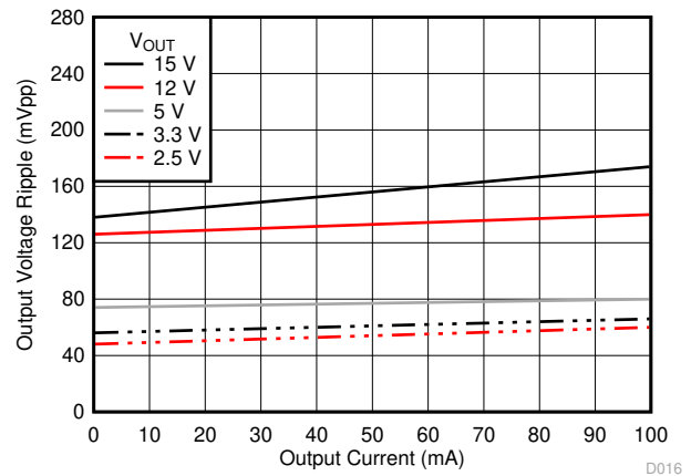
C_{OUT} = 47 \mu\text{F} , 16-V, ceramic Figure 6-14. Output Voltage Ripple
