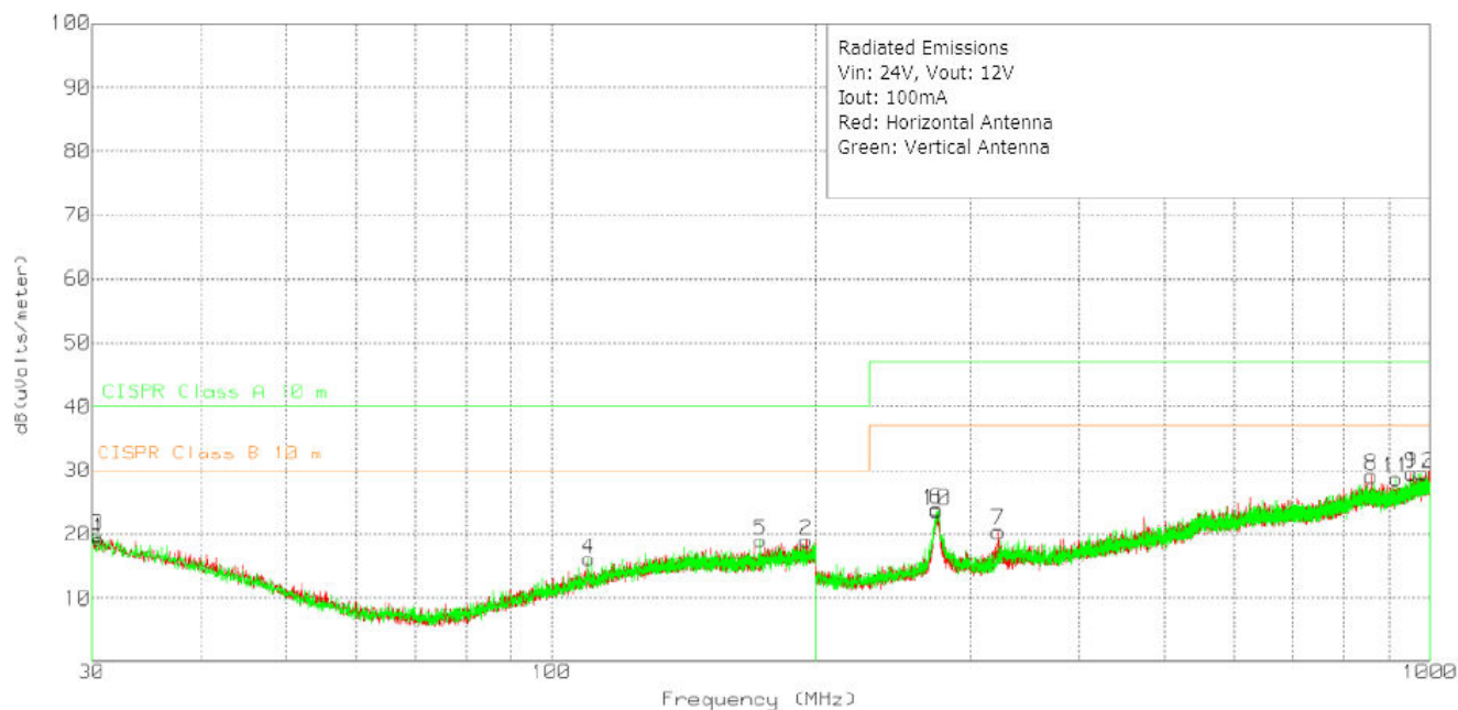
Figure 10-6. Radiated Emissions 24-V Input, 12-V Output, 100-mA Load
