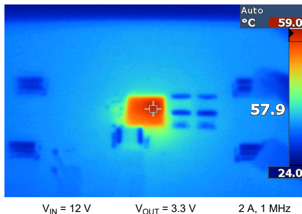
Figure 8-15. EVM Thermal Performance
