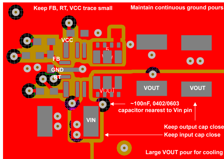
Figure 8-23. Example Layout
