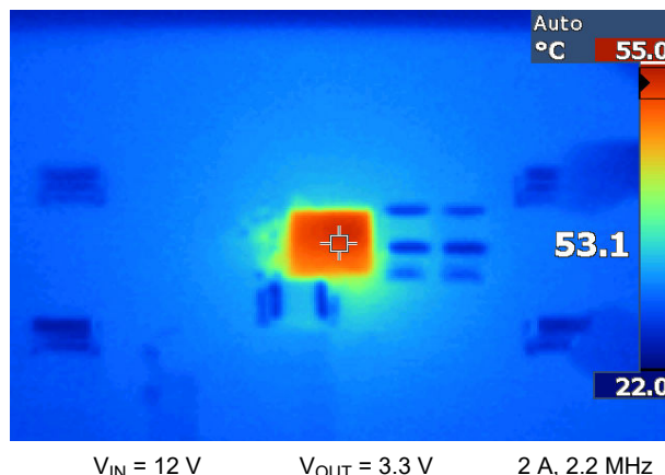
Figure 8-16. EVM Thermal Performance
