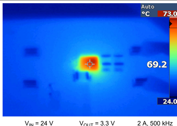
Figure 8-17. EVM Thermal Performance
