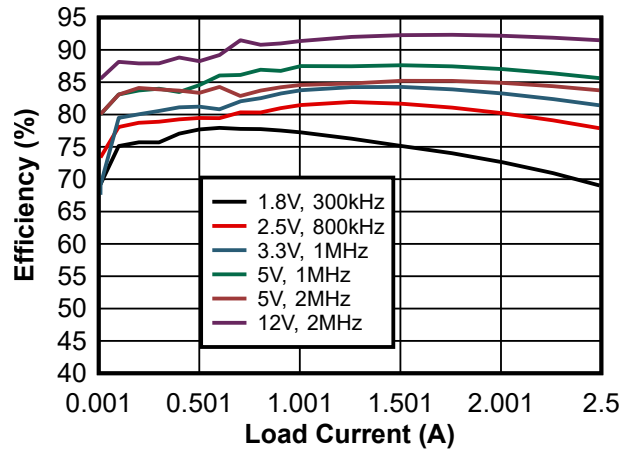
Figure 8-10. 36VIN Efficiency (Linear)
