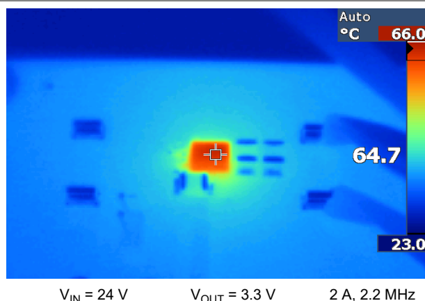
Figure 8-19. EVM Thermal Performance
