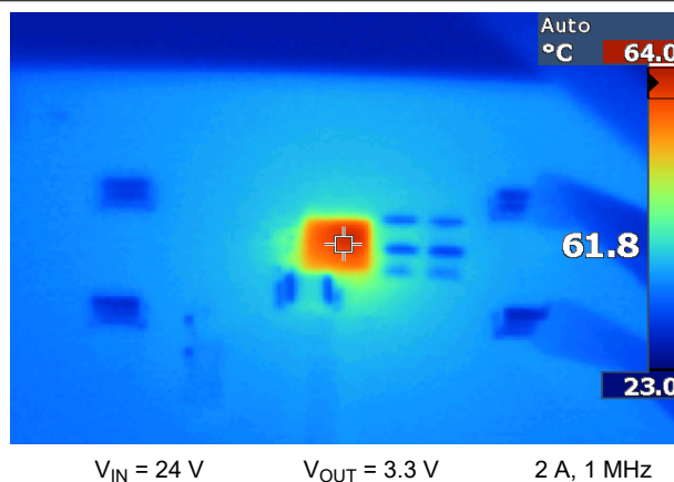
Figure 8-18. EVM Thermal Performance
