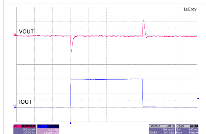
Figure 8-13. Load Transient, 12VIN, 3.3VOUT, 2.2MHz (FPWM), 0A to 2A, 1A/μs, COUT = 2x 22μF
