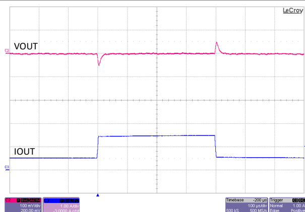
Figure 8-15. Load Transient, 12VIN, 3.3VOUT, 2.2MHz (FPWM), 0.5A to 1.5A, 1A/μs, COUT = 2x 22μF
