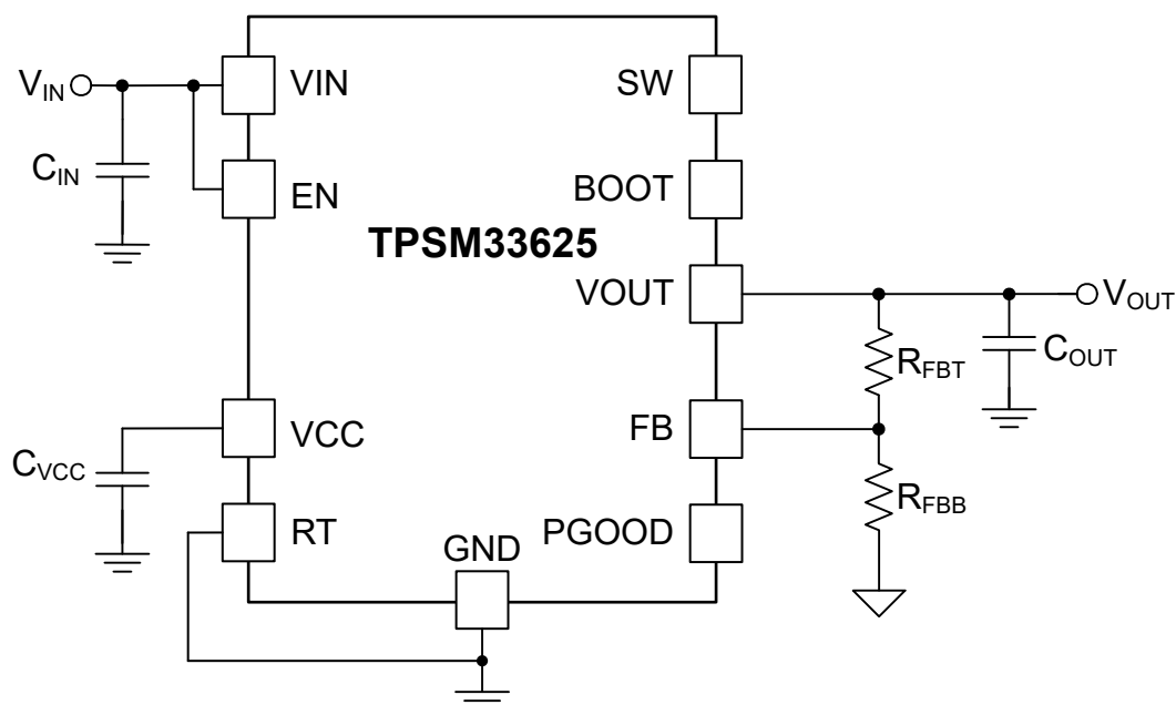
Typical Schematic
