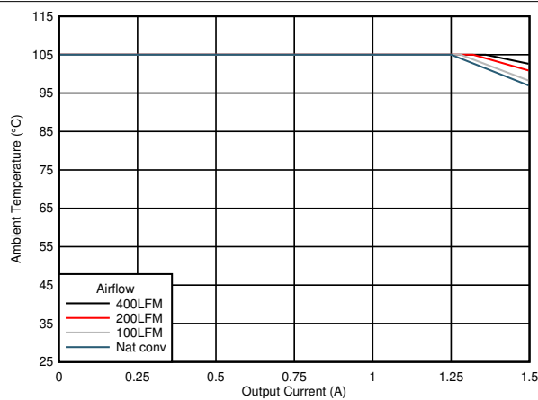
Figure 7-5. Safe Operating Area ( V_{OUT} = 3.3\text{ V} )
