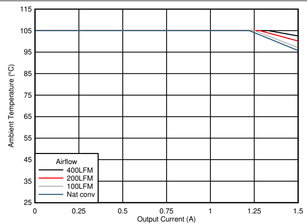
Figure 7-4. Safe Operating Area ( V_{OUT} = 1.2\text{ V} )
