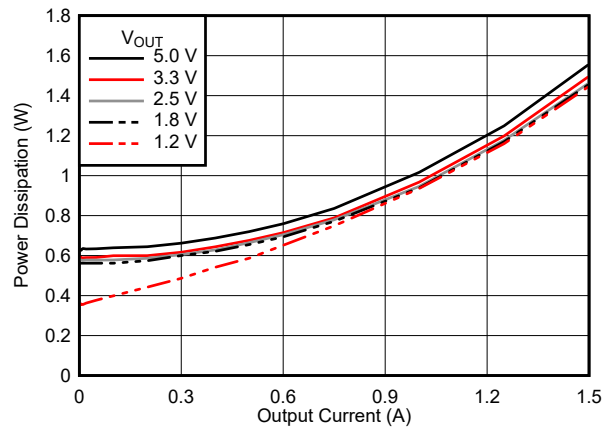
Figure 7-18. Power Dissipation
