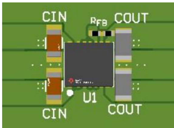
Figure 11-1. Typical Layout
