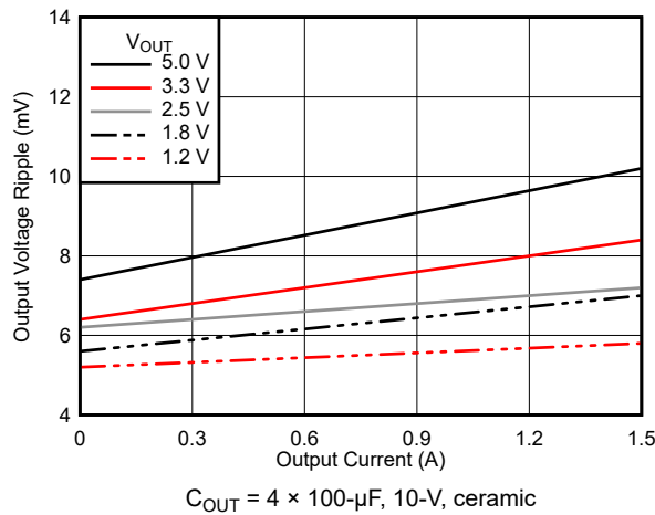
C_{OUT} = 4 \times 100\text{-}\mu\text{F} , 10-V, ceramic Figure 7-19. Output Voltage Ripple
