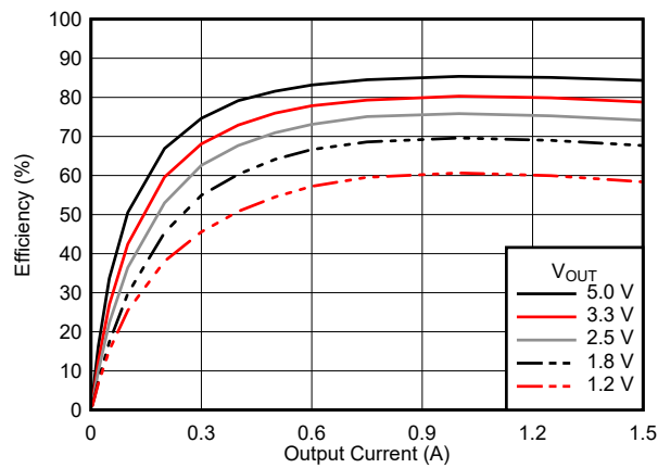
Figure 7-12. Efficiency
