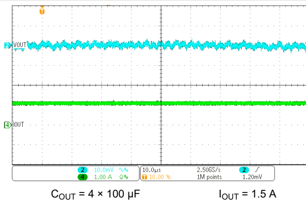
Figure 9-4. Output Ripple Waveform
