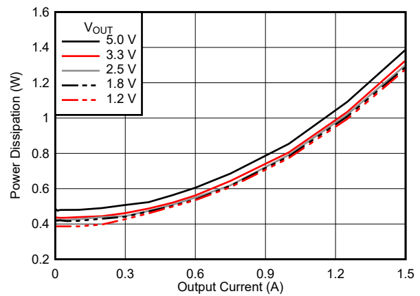
Figure 7-13. Power Dissipation
