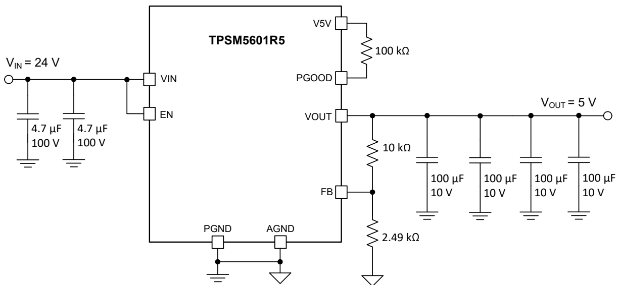
Figure 9-1. TPSM5601R5 Typical Schematic
