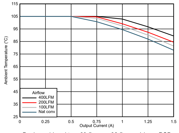
Device soldered to a 63.5-mm \times 82.5-mm, 4-layer PCB Figure 7-20. Safe Operating Area ( V_{OUT} = 3.3\text{ V} )
