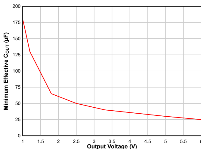
Figure 8-2. Minimum Required Output Capacitance
