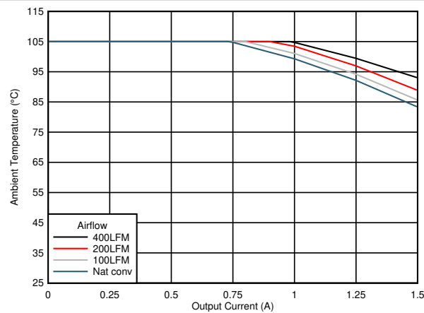
Figure 7-15. Safe Operating Area ( V_{OUT} = 3.3\text{ V} )
