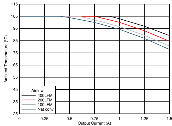
Device soldered to a 63.5-mm \times 82.5-mm, 4-layer PCB Figure 7-21. Safe Operating Area ( V_{OUT} = 5.0\text{ V} )
