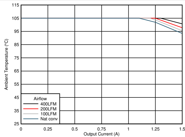
Figure 7-10. Safe Operating Area ( V_{OUT} = 1.8\text{ V} )
