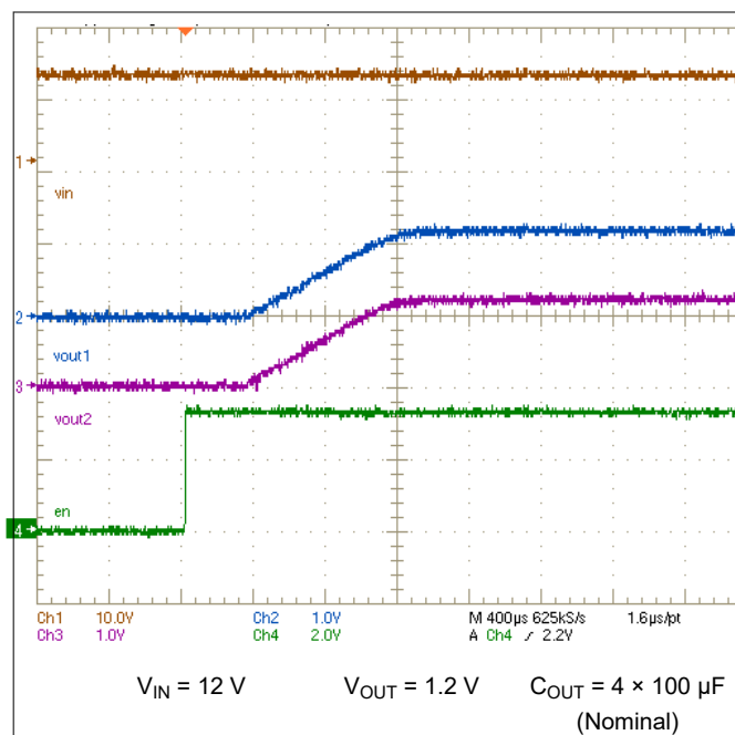
Figure 8-6. Enable Turn-On Without Load
