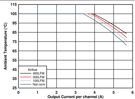
Figure 6-11. Safe Operating Area ( V_{OUT} = 0.8\text{ V} )
