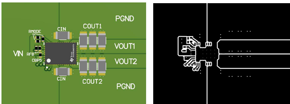
Figure 10-1. Typical Dual-Output Layout
