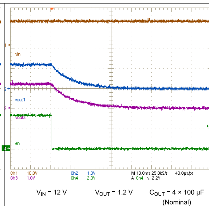
Figure 8-7. Enable Turn-Off Without Load
