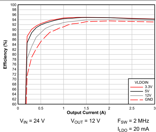
Figure 7-9. Efficiency improvements with VLDOIN (VOUT = 12 V)
