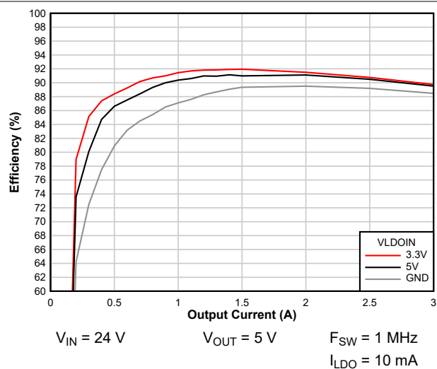
Figure 7-8. Efficiency improvements with VLDOIN (VOUT = 5 V)
