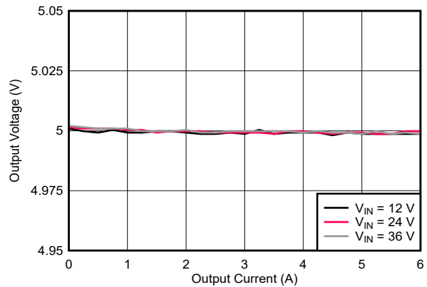
Figure 9-3. Load Regulation
