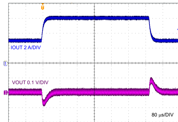
Figure 9-6. Load Transient, 3 A to 6 A, 1 A/ \mu\text{s}
