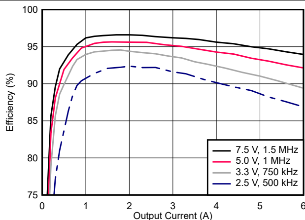
Figure 7-9. Efficiency
