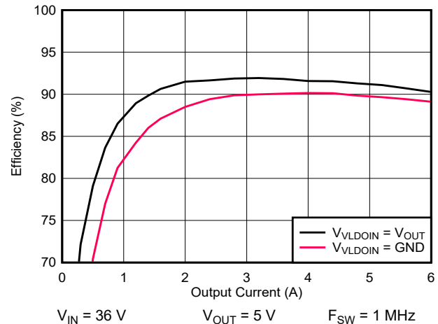
Figure 8-6. Efficiency Increase With External Bias
