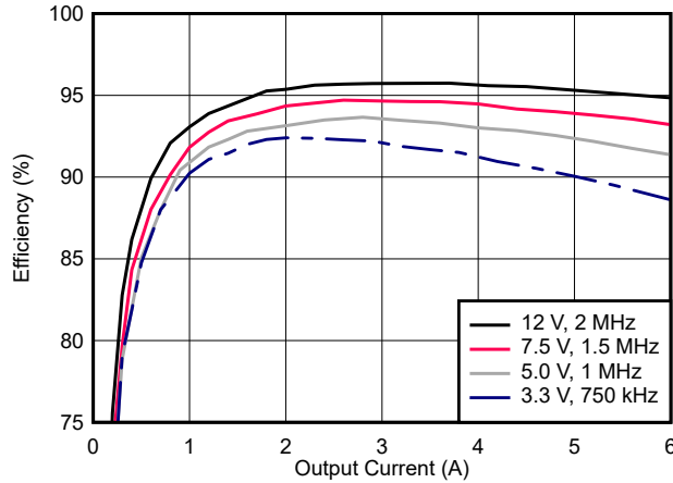
Figure 7-14. Efficiency
