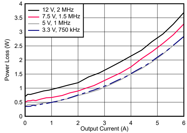
Figure 7-15. Power Dissipation
