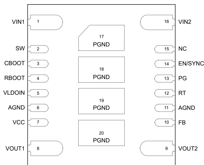
Figure 6-1. 20-Pin QFN RDL Package (Top View)
