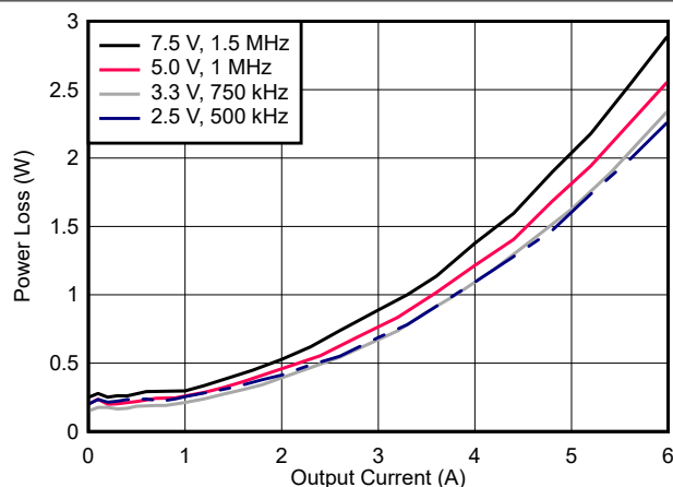
Figure 7-10. Power Dissipation
