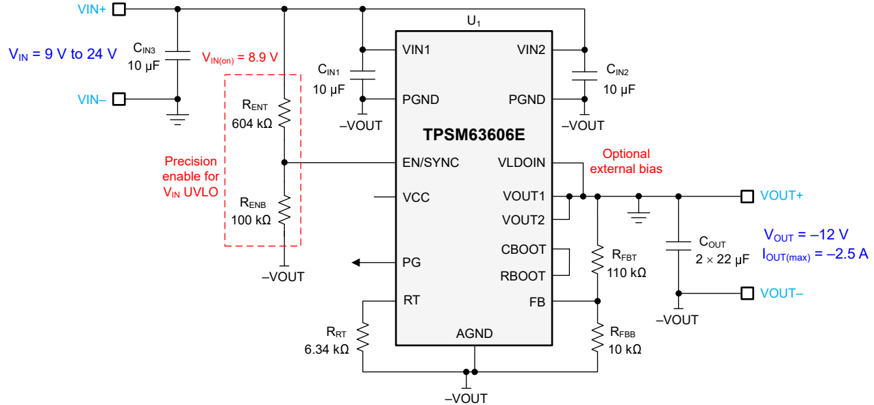
Figure 9-12. Circuit Schematic
