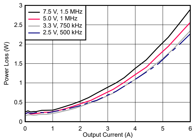
Figure 7-10. Power Dissipation
