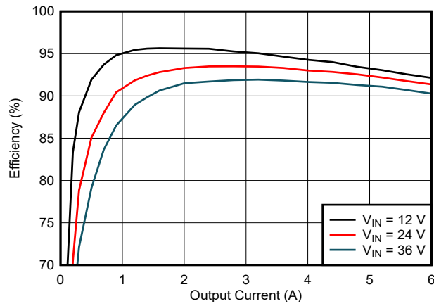
Figure 9-2. Efficiency
