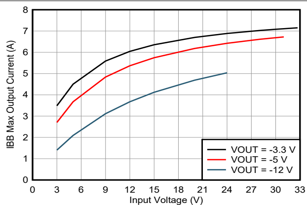
Figure 9-15. IBB Maximum Output Current
