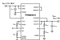
Typical Schematic
