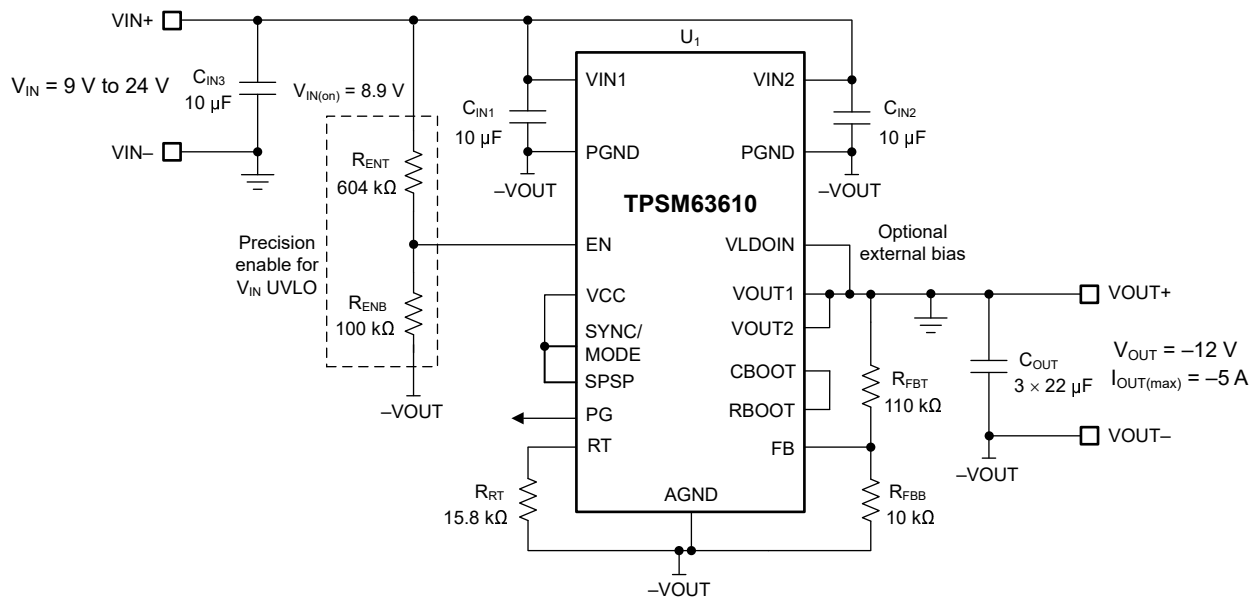
Figure 9-14. Circuit Schematic
