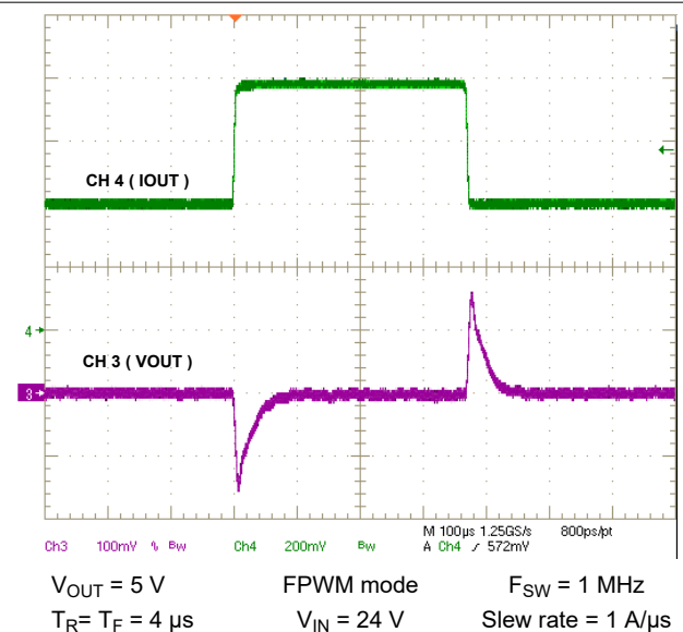
Figure 9-7. Load Transient, 4 A to 8 A, 1 A/μs
