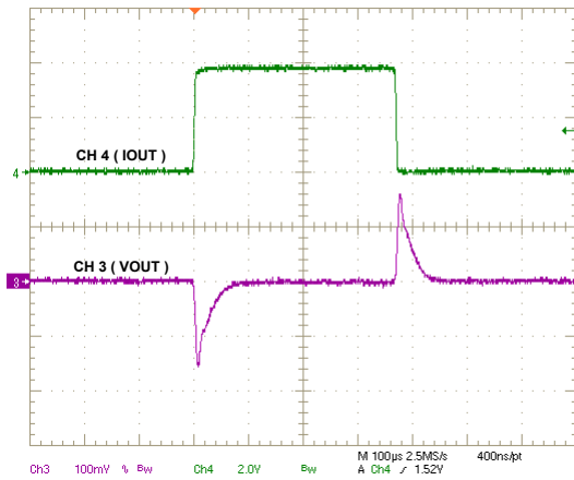
Figure 9-8. Load Transient, 0 A to 4 A, 1 A/μs
