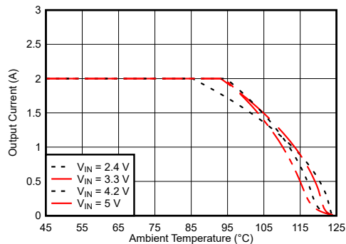
Figure 9-94. Safe Operating Area
