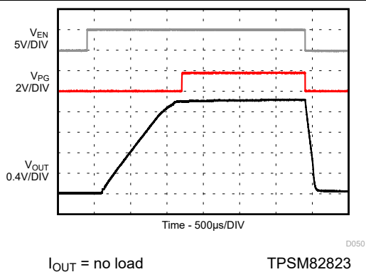
Figure 9-133. Start-up / Shutdown without Load
