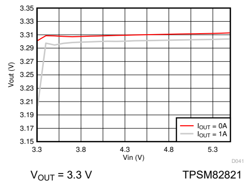
Figure 9-24. Line Regulation
