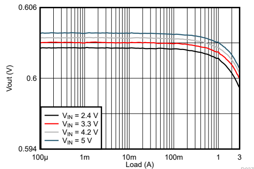
Figure 9-150. Load Regulation
