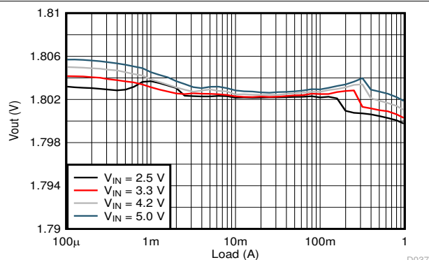
Figure 9-18. Load Regulation
