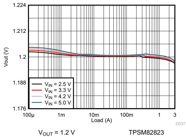
Figure 9-124. Load Regulation
