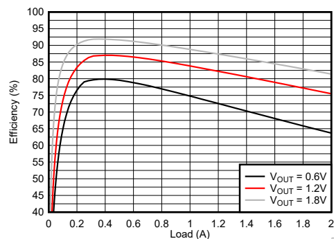
Figure 9-93. Efficiency
