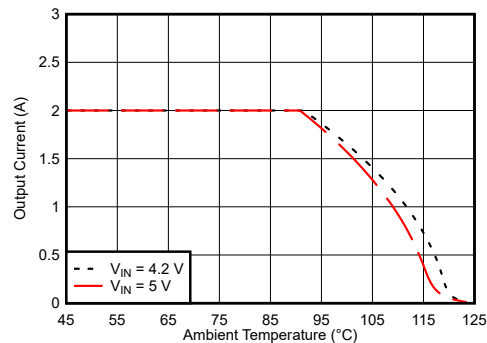
Figure 9-95. Safe Operating Area
