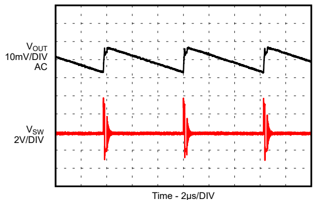
Figure 9-129. Output Ripple in PSM Mode
