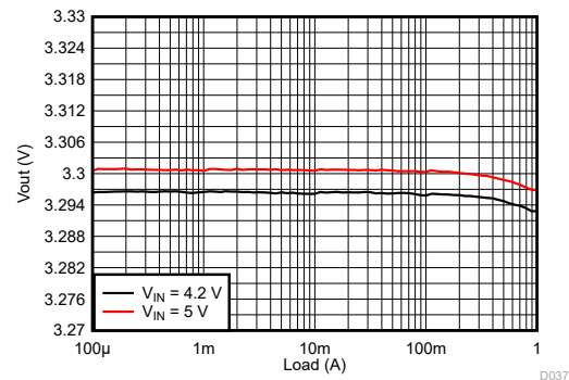
Figure 9-44. Load Regulation
