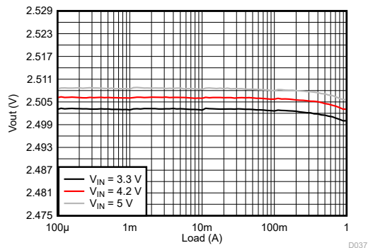
Figure 9-43. Load Regulation
