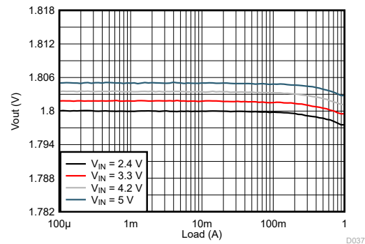
Figure 9-42. Load Regulation
