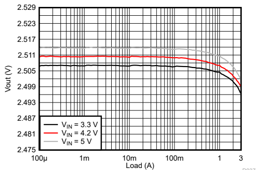
Figure 9-151. Load Regulation
