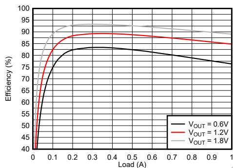
Figure 9-92. Efficiency
