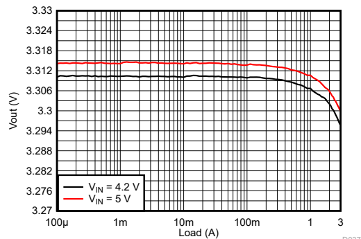
Figure 9-152. Load Regulation
