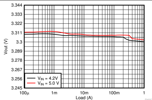
Figure 9-18. Load Regulation
