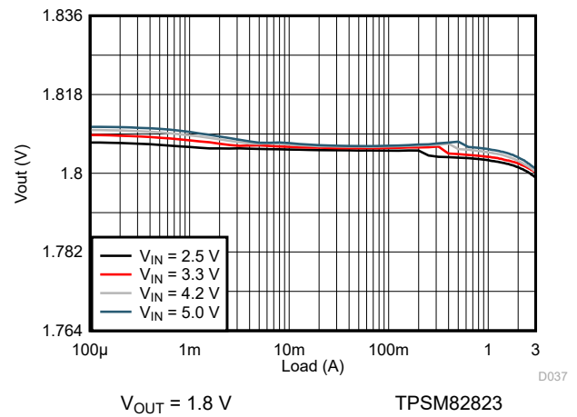
Figure 9-125. Load Regulation
