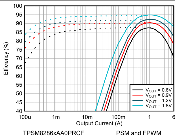
Figure 8-6. Efficiency V_{IN} = 2.8\text{ V} and T_A = 25^\circ\text{C}
