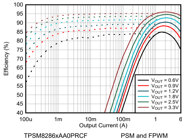
Figure 8-2. Efficiency V_{IN} = 5.0\text{ V} and T_A = 25^\circ\text{C}
