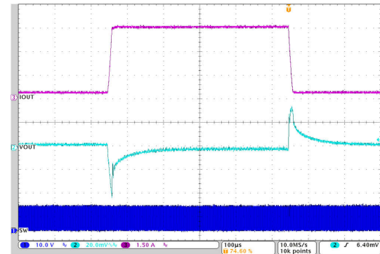
Figure 7-17. Load Transient
