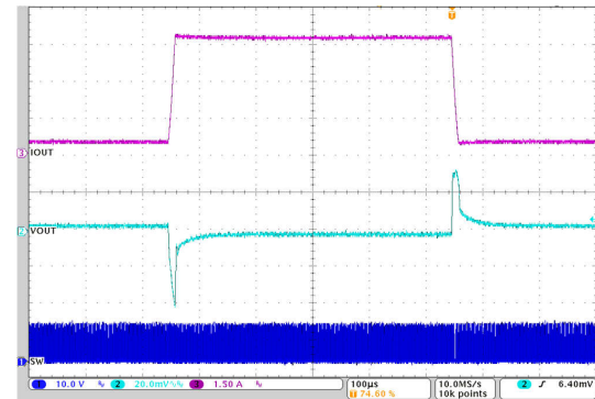
Figure 7-15. Load Transient
