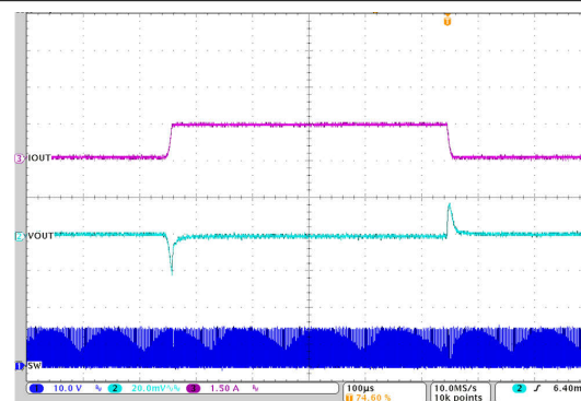
Figure 7-11. Load Transient
