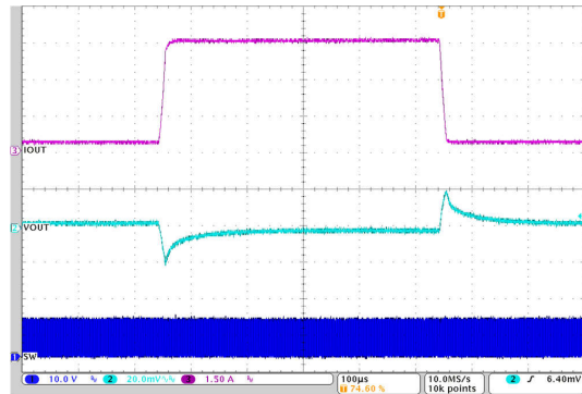
Figure 7-16. Load Transient
