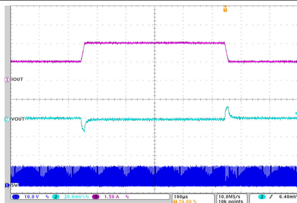
Figure 7-10. Load Transient
