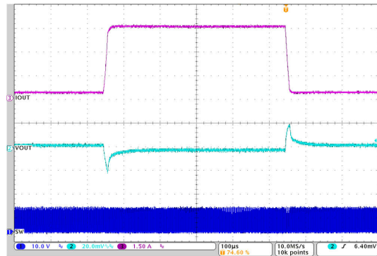
Figure 7-14. Load Transient
