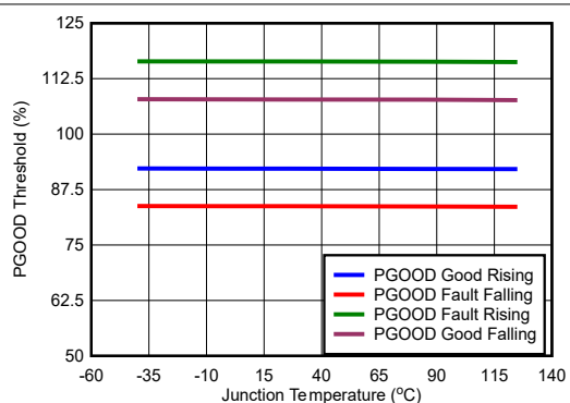
Figure 5-9. PG Threshold
