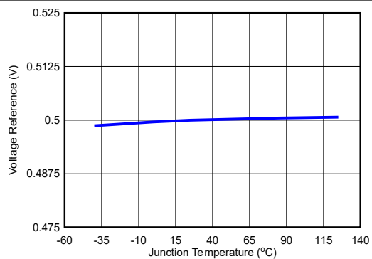
Figure 5-7. Voltage Reference
