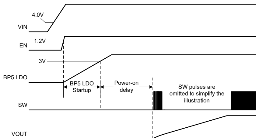
Figure 6-1. Start-Up Sequence
