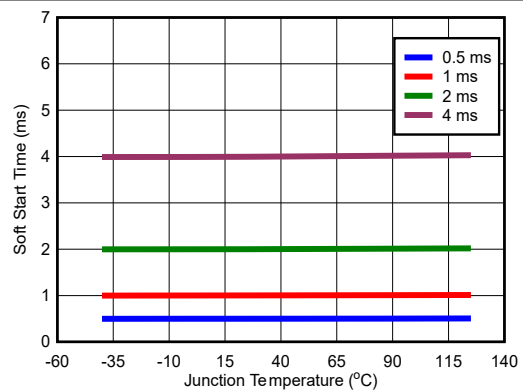
Figure 5-11. Soft Start
