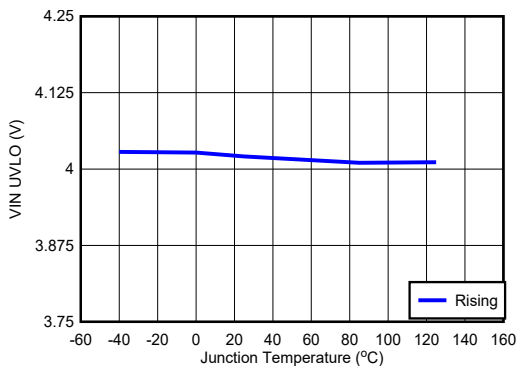
Figure 6-7. V_{IN} UVLO
