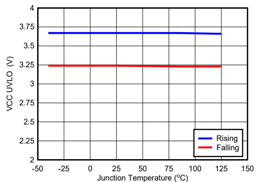
Figure 6-8. V_{CC} UVLO
