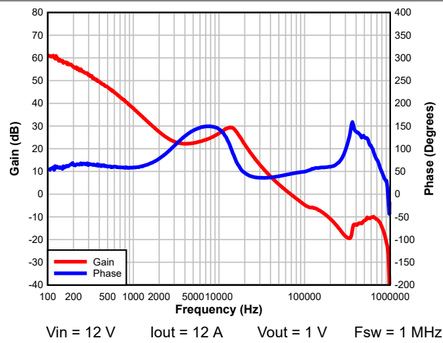
Figure 8-7. Bode Plot
